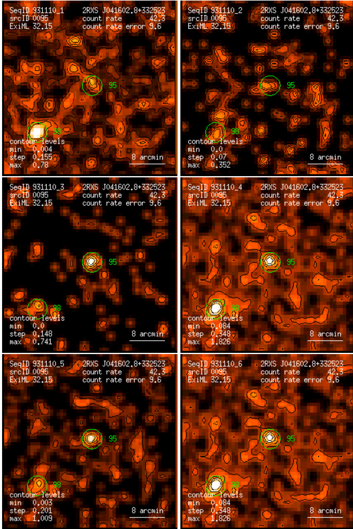
Figure 95: RASS 931110: detection 0095: band rate images, Gaussian filter: (1) PSPC channels 11 – 41, (2) 52 – 90, (3) 91 – 201, (4) 11 – 235, (5) 52 – 201, (6) 11 – 201. Broad band rates in counts/ks. Band rate contour levels in counts/ks/arcmin 2 .
