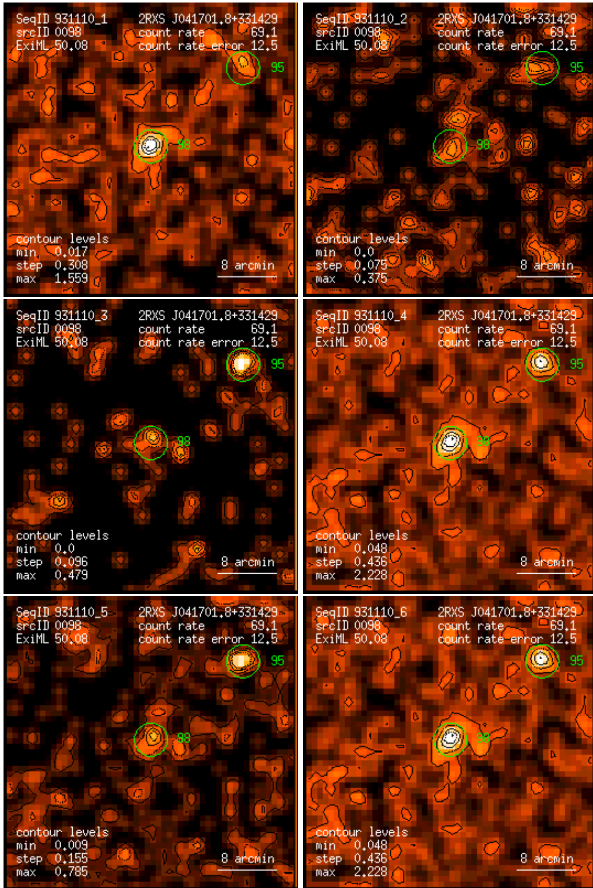
Figure 98: RASS 931110: detection 0098: band rate images, Gaussian filter: (1) PSPC channels 11 – 41, (2) 52 – 90, (3) 91 – 201, (4) 11 – 235, (5) 52 – 201, (6) 11 – 201. Broad band rates in counts/ks. Band rate contour levels in counts/ks/arcmin 2 .
