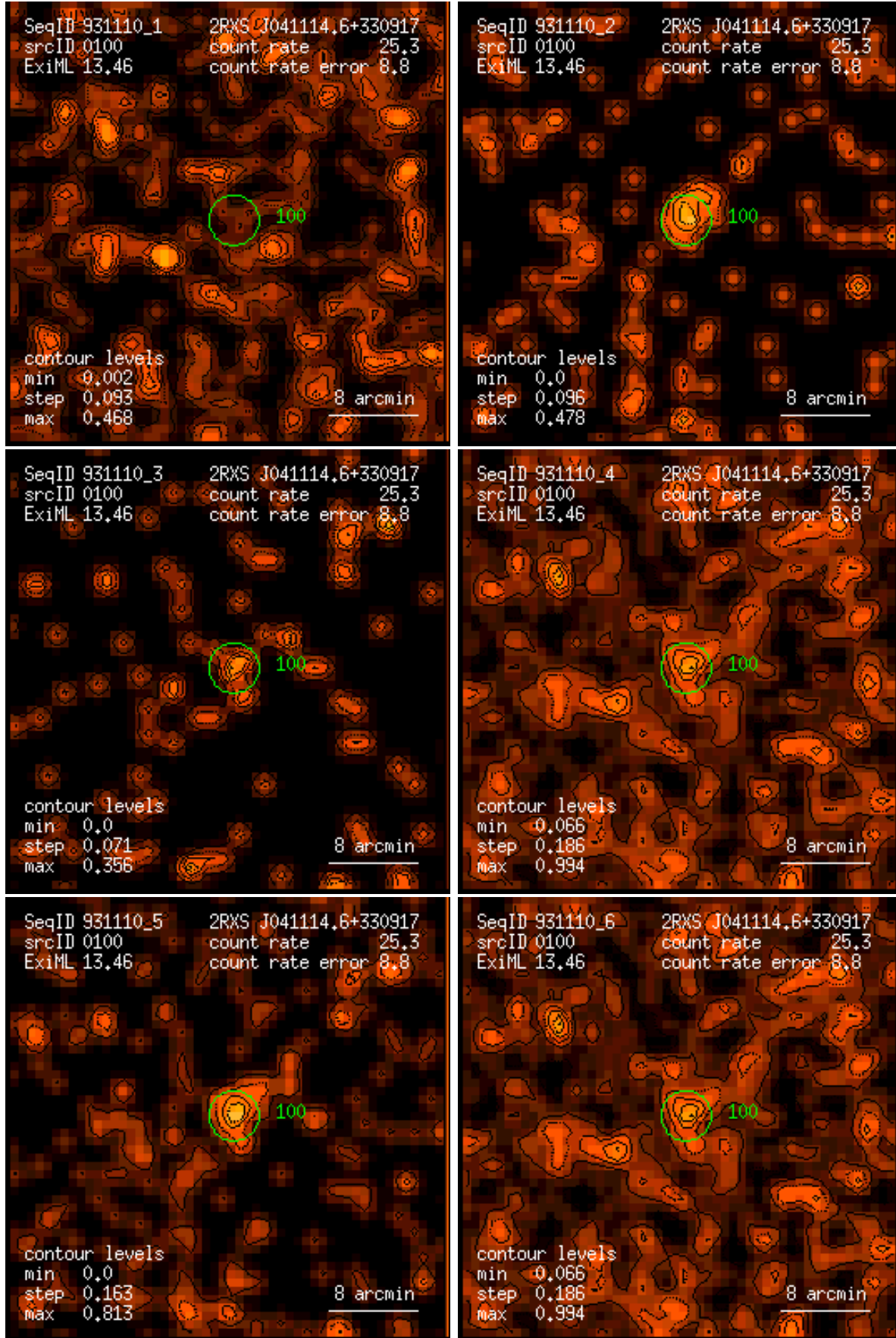
Figure 100: RASS 931110: detection 0100: band rate images, Gaussian filter: (1) PSPC channels 11 – 41, (2) 52 – 90, (3) 91 – 201, (4) 11 – 235, (5) 52 – 201, (6) 11 – 201. Broad band rates in counts/ks. Band rate contour levels in counts/ks/arcmin 2 .
