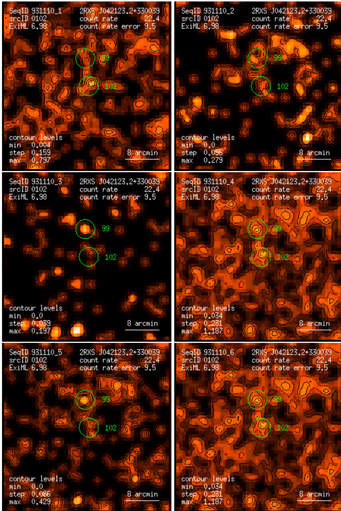
Figure 102: RASS 931110: detection 0102: band rate images, Gaussian filter: (1) PSPC channels 11 – 41, (2) 52 – 90, (3) 91 – 201, (4) 11 – 235, (5) 52 – 201, (6) 11 – 201. Broad band rates in counts/ks. Band rate contour levels in counts/ks/arcmin 2 .
