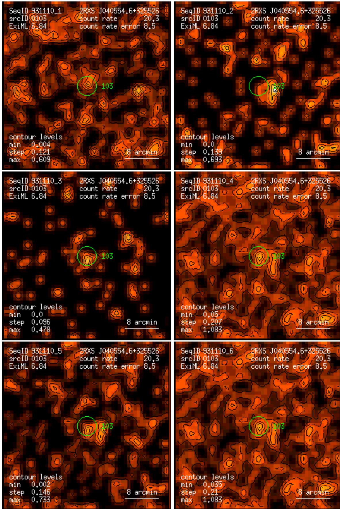
Figure 103: RASS 931110: detection 0103: band rate images, Gaussian filter: (1) PSPC channels 11 – 41, (2) 52 – 90, (3) 91 – 201, (4) 11 – 235, (5) 52 – 201, (6) 11 – 201. Broad band rates in counts/ks. Band rate contour levels in counts/ks/arcmin 2 .
