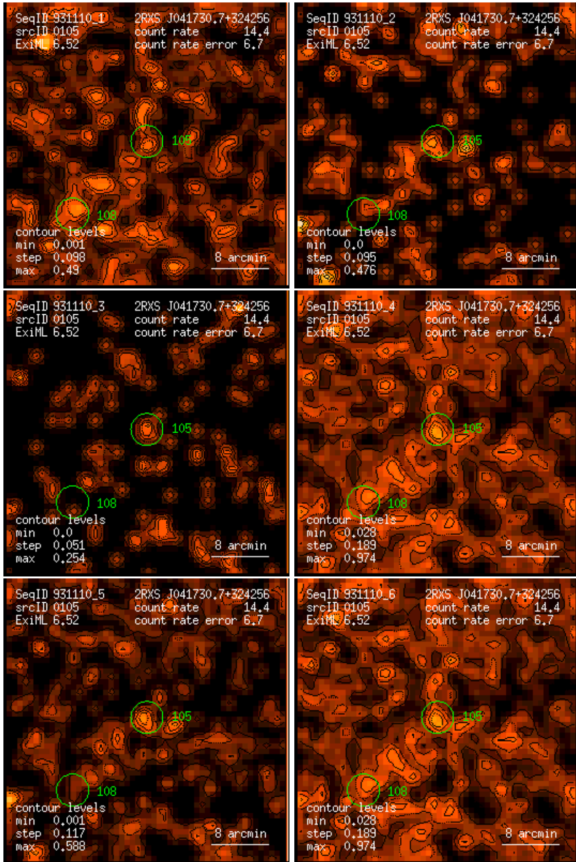
Figure 105: RASS 931110: detection 0105: band rate images, Gaussian filter: (1) PSPC channels 11 – 41, (2) 52 – 90, (3) 91 – 201, (4) 11 – 235, (5) 52 – 201, (6) 11 – 201. Broad band rates in counts/ks. Band rate contour levels in counts/ks/arcmin 2 .
