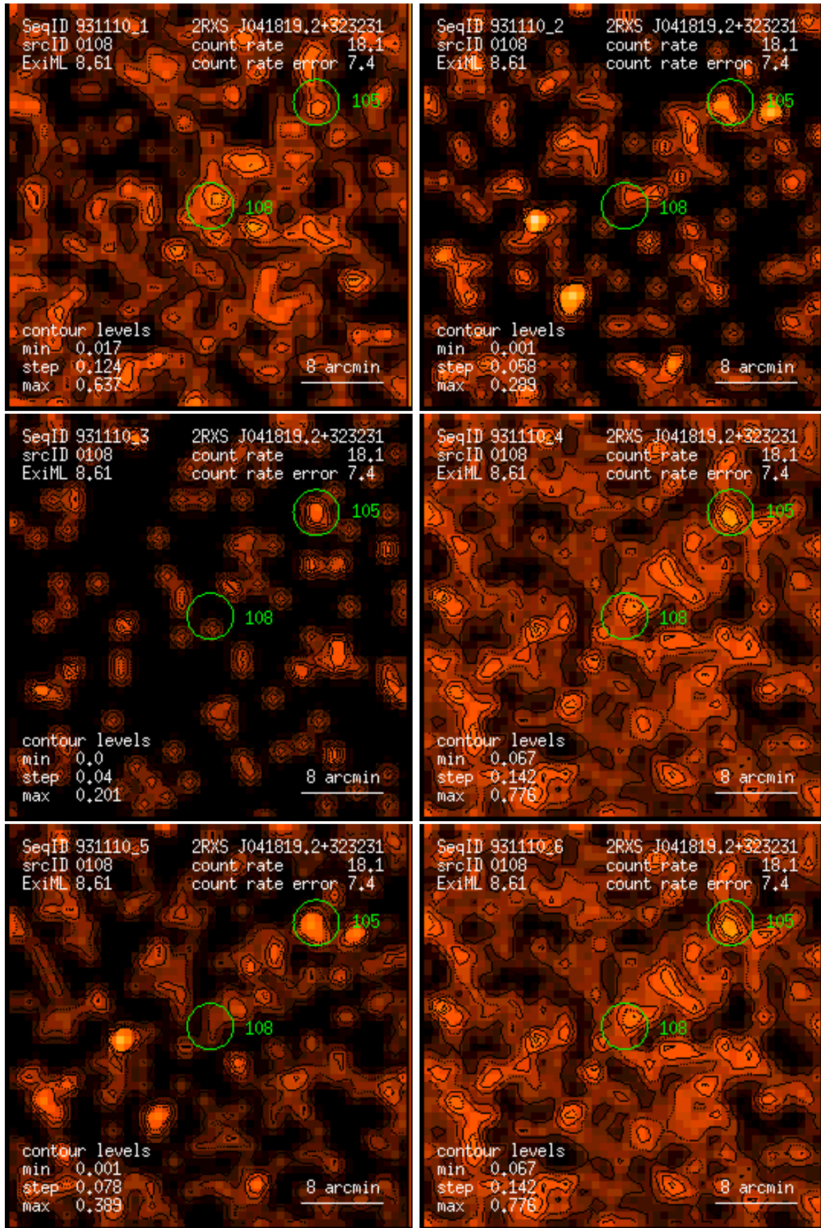
Figure 108: RASS 931110: detection 0108: band rate images, Gaussian filter: (1) PSPC channels 11 – 41, (2) 52 – 90, (3) 91 – 201, (4) 11 – 235, (5) 52 – 201, (6) 11 – 201. Broad band rates in counts/ks. Band rate contour levels in counts/ks/arcmin 2 .
