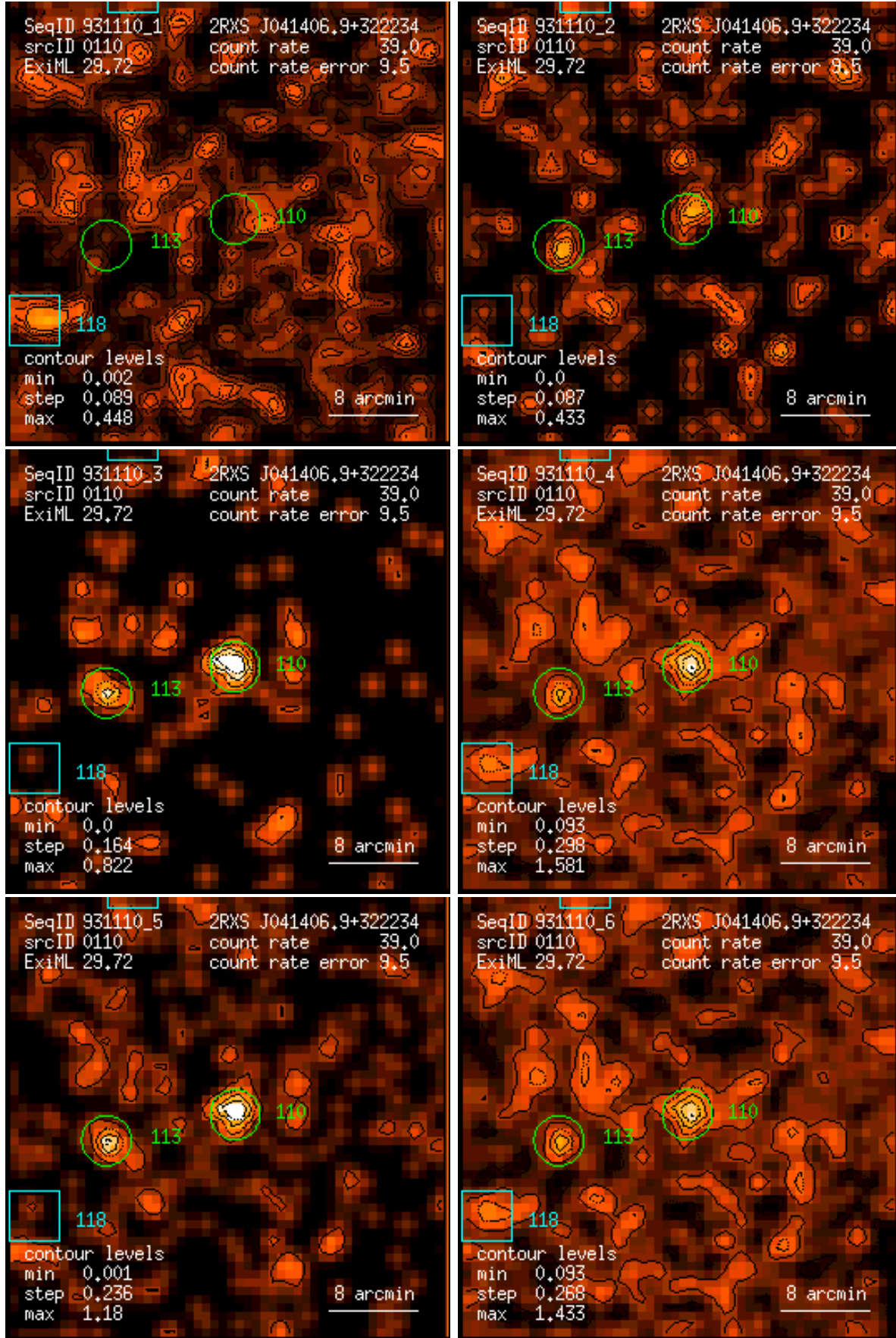
Figure 110: RASS 931110: detection 0110: band rate images, Gaussian filter: (1) PSPC channels 11 – 41, (2) 52 – 90, (3) 91 – 201, (4) 11 – 235, (5) 52 – 201, (6) 11 – 201. Broad band rates in counts/ks. Band rate contour levels in counts/ks/arcmin 2 .
