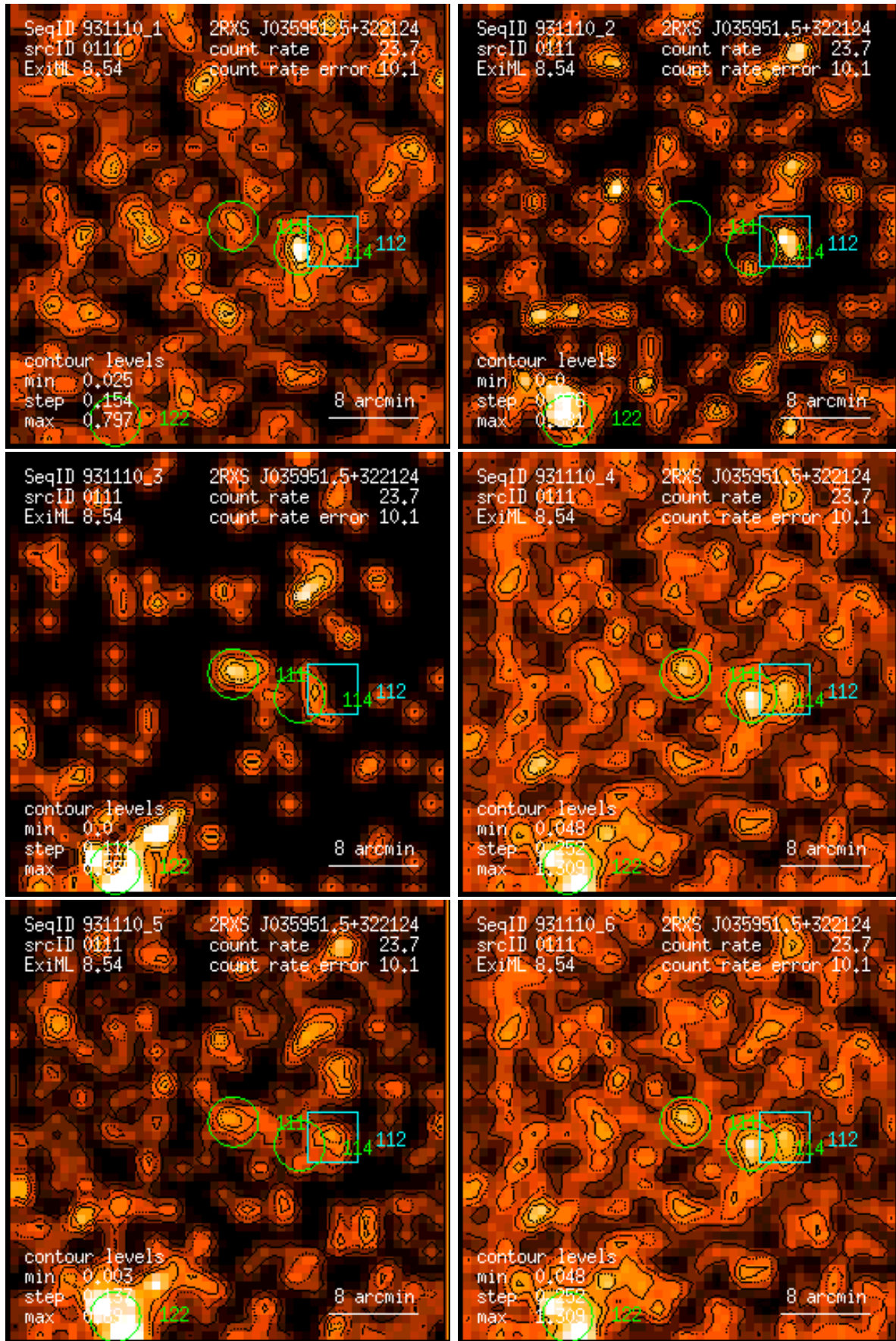
Figure 111: RASS 931110: detection 0111: band rate images, Gaussian filter: (1) PSPC channels 11 – 41, (2) 52 – 90, (3) 91 – 201, (4) 11 – 235, (5) 52 – 201, (6) 11 – 201. Broad band rates in counts/ks. Band rate contour levels in counts/ks/arcmin 2 .
