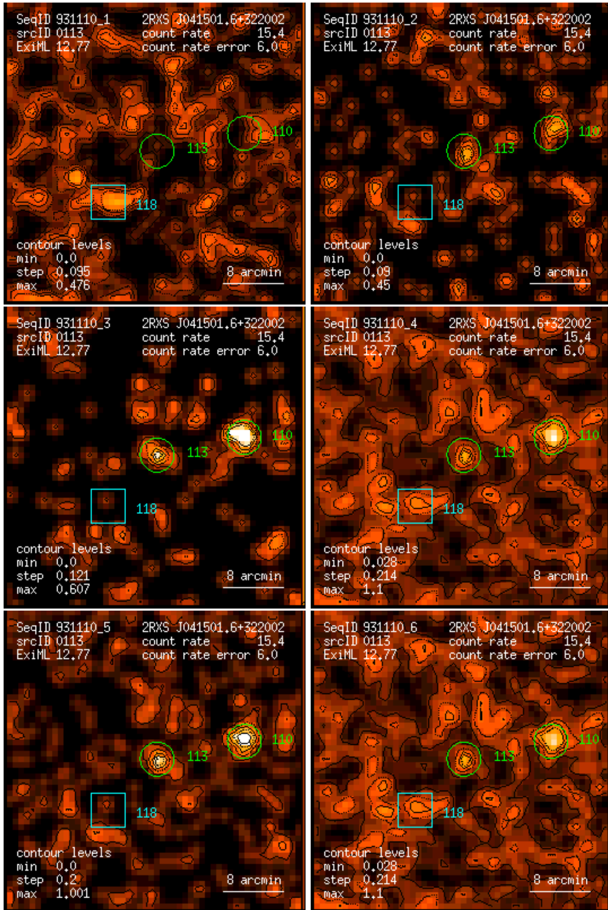
Figure 113: RASS 931110: detection 0113: band rate images, Gaussian filter: (1) PSPC channels 11 – 41, (2) 52 – 90, (3) 91 – 201, (4) 11 – 235, (5) 52 – 201, (6) 11 – 201. Broad band rates in counts/ks. Band rate contour levels in counts/ks/arcmin 2 .
