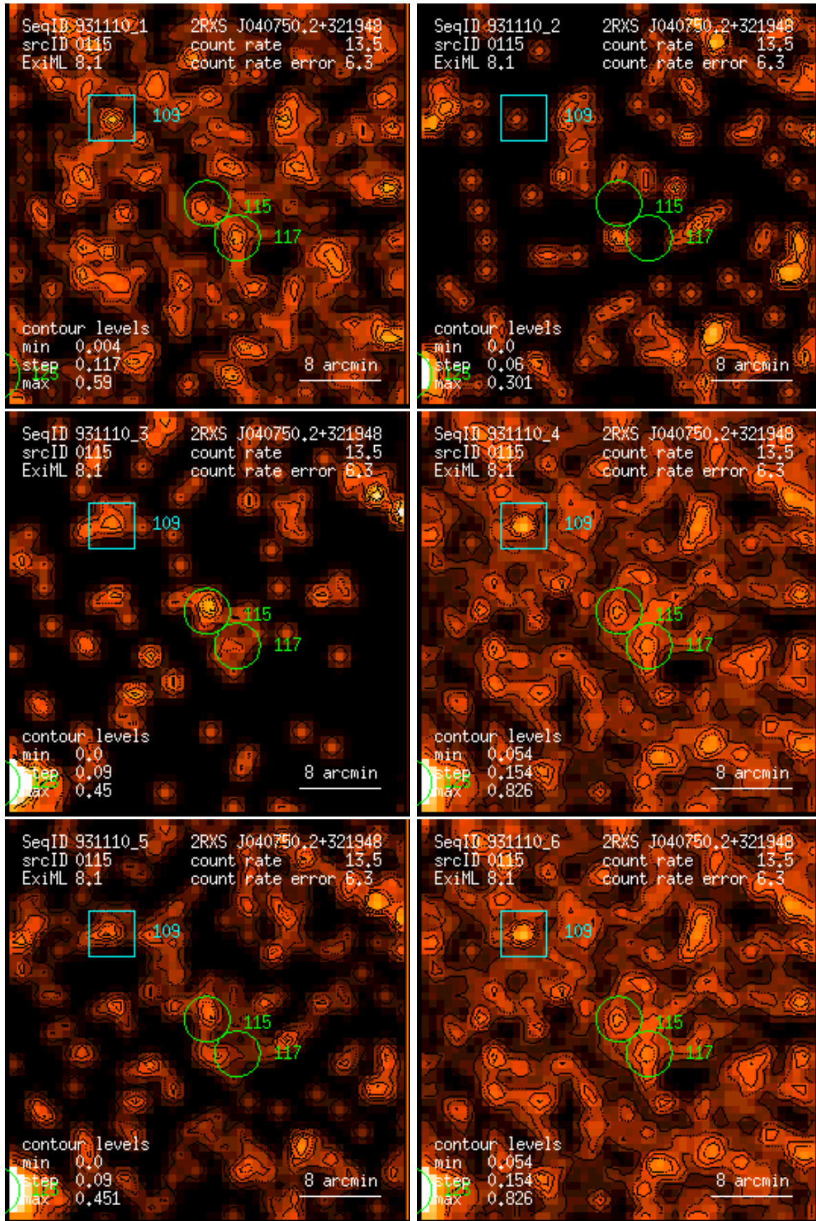
Figure 115: RASS 931110: detection 0115: band rate images, Gaussian filter: (1) PSPC channels 11 – 41, (2) 52 – 90, (3) 91 – 201, (4) 11 – 235, (5) 52 – 201, (6) 11 – 201. Broad band rates in counts/ks. Band rate contour levels in counts/ks/arcmin 2 .
