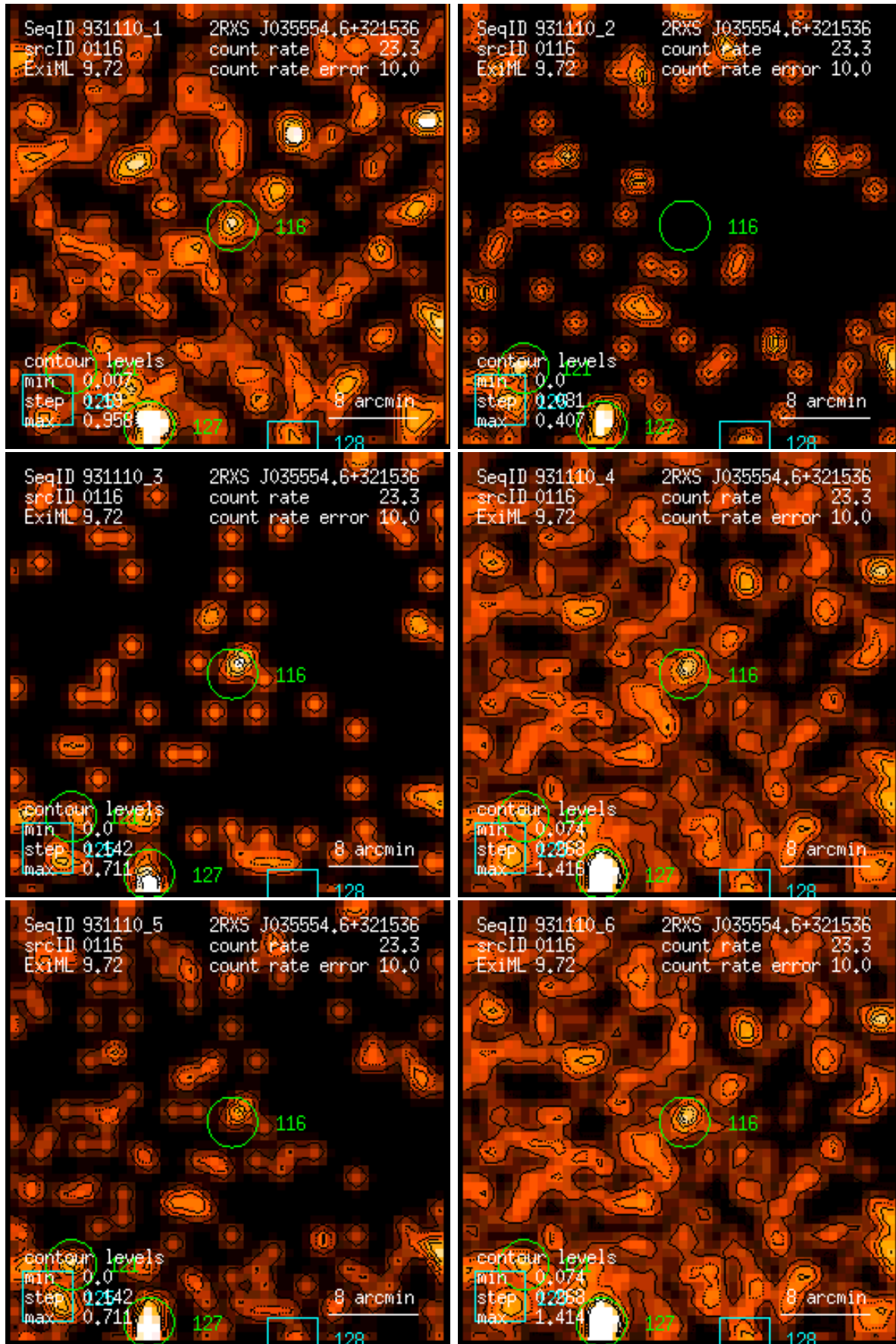
Figure 116: RASS 931110: detection 0116: band rate images, Gaussian filter: (1) PSPC channels 11 – 41, (2) 52 – 90, (3) 91 – 201, (4) 11 – 235, (5) 52 – 201, (6) 11 – 201. Broad band rates in counts/ks. Band rate contour levels in counts/ks/arcmin 2 .
