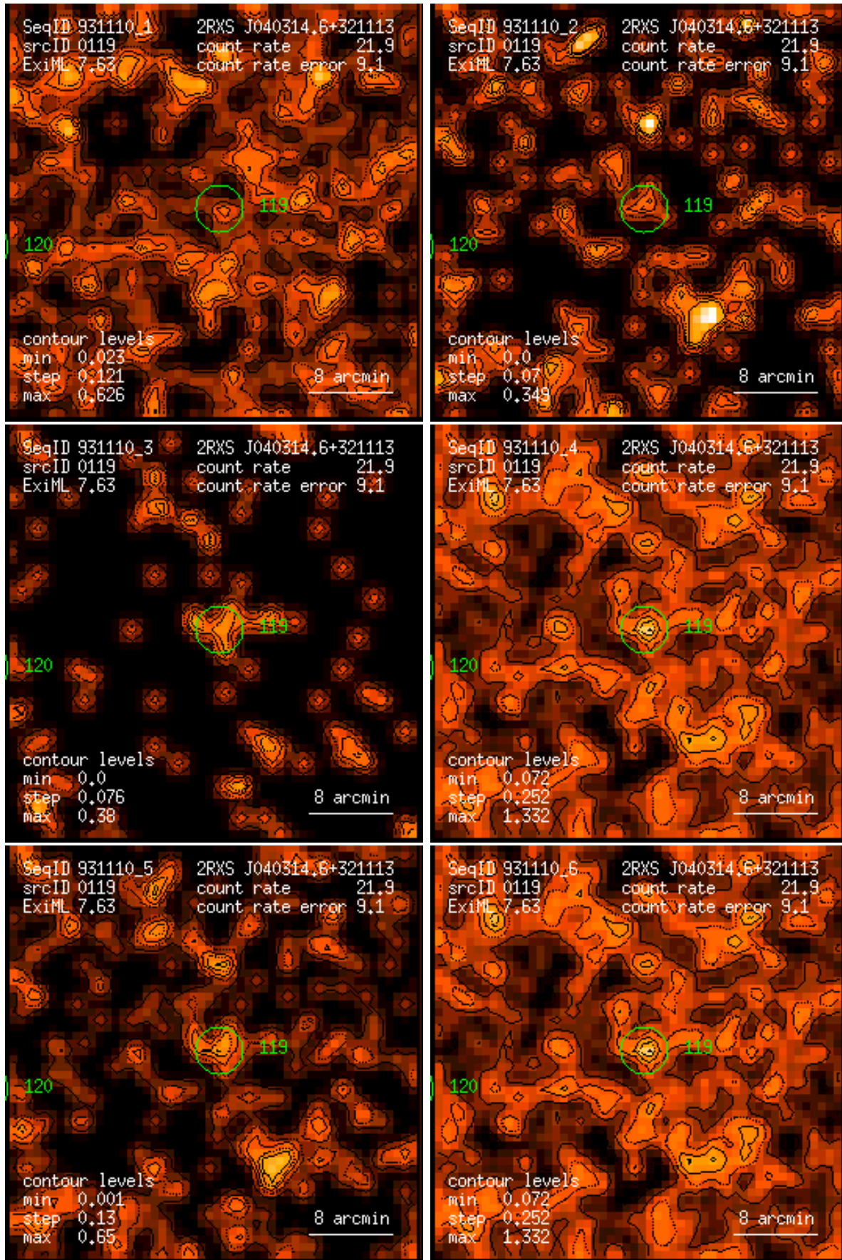
Figure 119: RASS 931110: detection 0119: band rate images, Gaussian filter: (1) PSPC channels 11 – 41, (2) 52 – 90, (3) 91 – 201, (4) 11 – 235, (5) 52 – 201, (6) 11 – 201. Broad band rates in counts/ks. Band rate contour levels in counts/ks/arcmin 2 .
