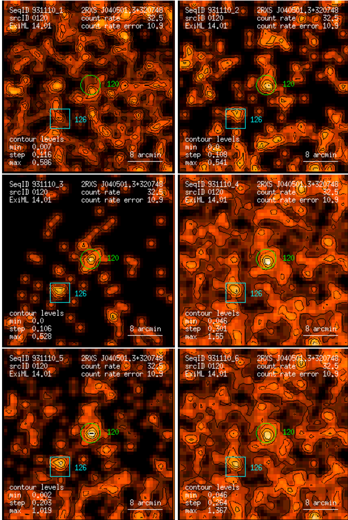
Figure 120: RASS 931110: detection 0120: band rate images, Gaussian filter: (1) PSPC channels 11 – 41, (2) 52 – 90, (3) 91 – 201, (4) 11 – 235, (5) 52 – 201, (6) 11 – 201. Broad band rates in counts/ks. Band rate contour levels in counts/ks/arcmin 2 .
