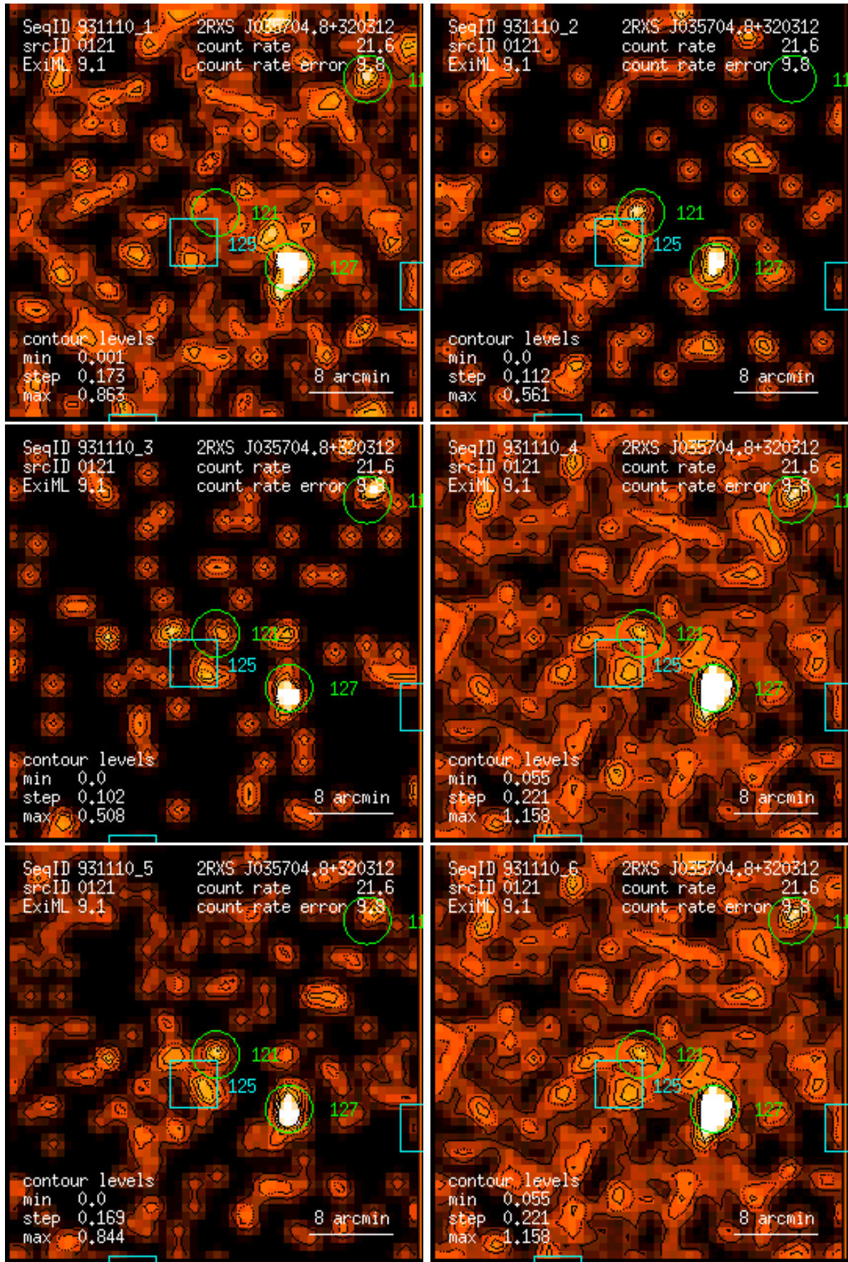
Figure 121: RASS 931110: detection 0121: band rate images, Gaussian filter: (1) PSPC channels 11 – 41, (2) 52 – 90, (3) 91 – 201, (4) 11 – 235, (5) 52 – 201, (6) 11 – 201. Broad band rates in counts/ks. Band rate contour levels in counts/ks/arcmin 2 .
