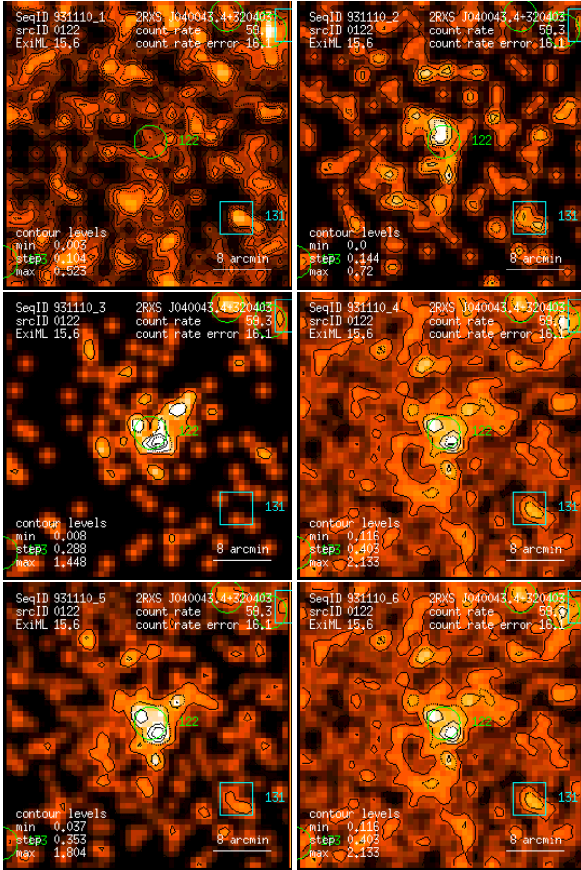
Figure 122: RASS 931110: detection 0122: band rate images, Gaussian filter: (1) PSPC channels 11 – 41, (2) 52 – 90, (3) 91 – 201, (4) 11 – 235, (5) 52 – 201, (6) 11 – 201. Broad band rates in counts/ks. Band rate contour levels in counts/ks/arcmin 2 .
