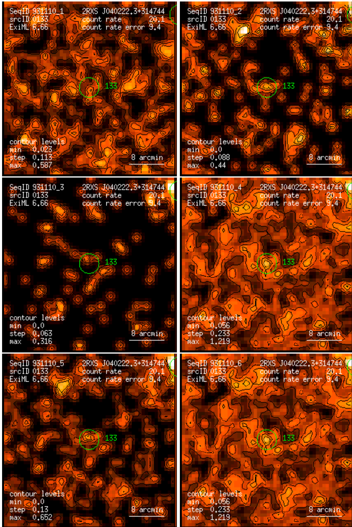
Figure 133: RASS 931110: detection 0133: band rate images, Gaussian filter: (1) PSPC channels 11 – 41, (2) 52 – 90, (3) 91 – 201, (4) 11 – 235, (5) 52 – 201, (6) 11 – 201. Broad band rates in counts/ks. Band rate contour levels in counts/ks/arcmin 2 .
