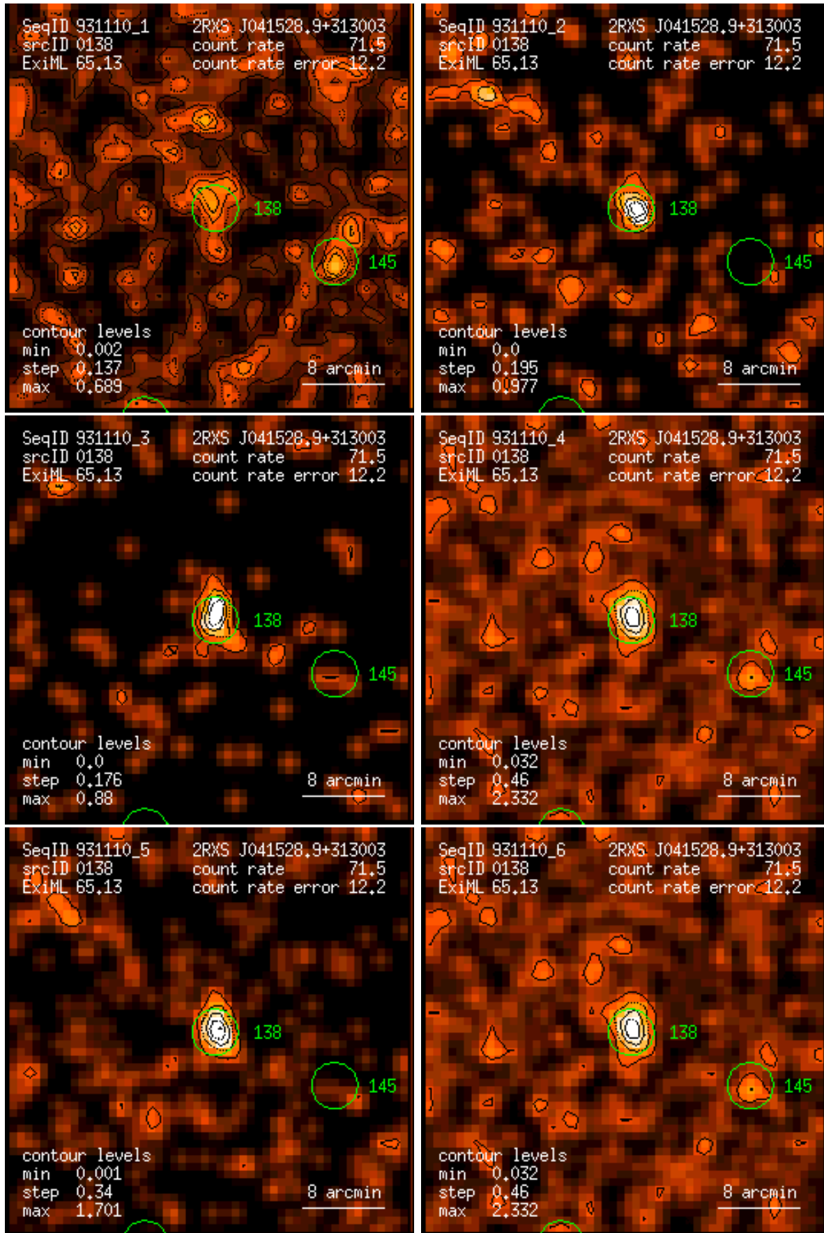
Figure 138: RASS 931110: detection 0138: band rate images, Gaussian filter: (1) PSPC channels 11 – 41, (2) 52 – 90, (3) 91 – 201, (4) 11 – 235, (5) 52 – 201, (6) 11 – 201. Broad band rates in counts/ks. Band rate contour levels in counts/ks/arcmin 2 .
