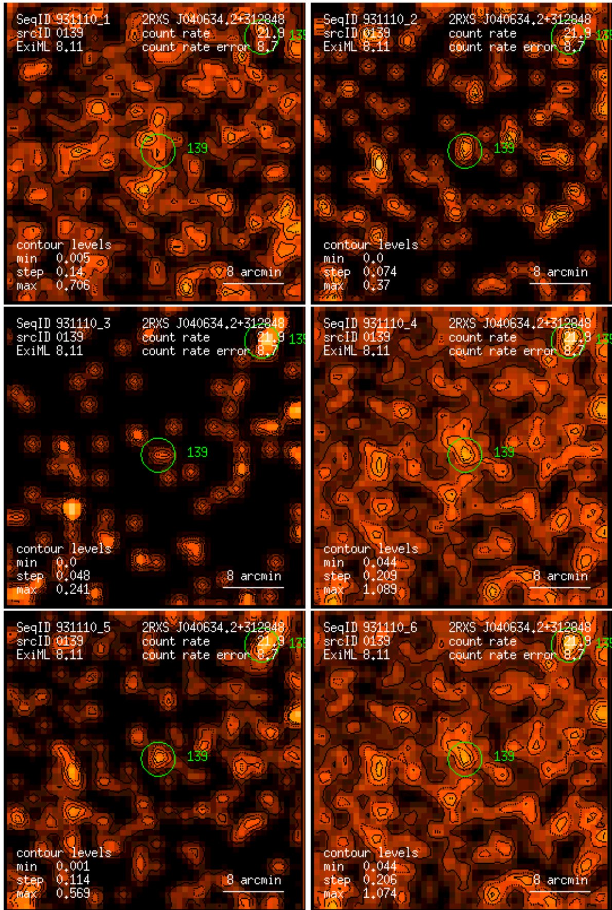
Figure 139: RASS 931110: detection 0139: band rate images, Gaussian filter: (1) PSPC channels 11 – 41, (2) 52 – 90, (3) 91 – 201, (4) 11 – 235, (5) 52 – 201, (6) 11 – 201. Broad band rates in counts/ks. Band rate contour levels in counts/ks/arcmin 2 .
