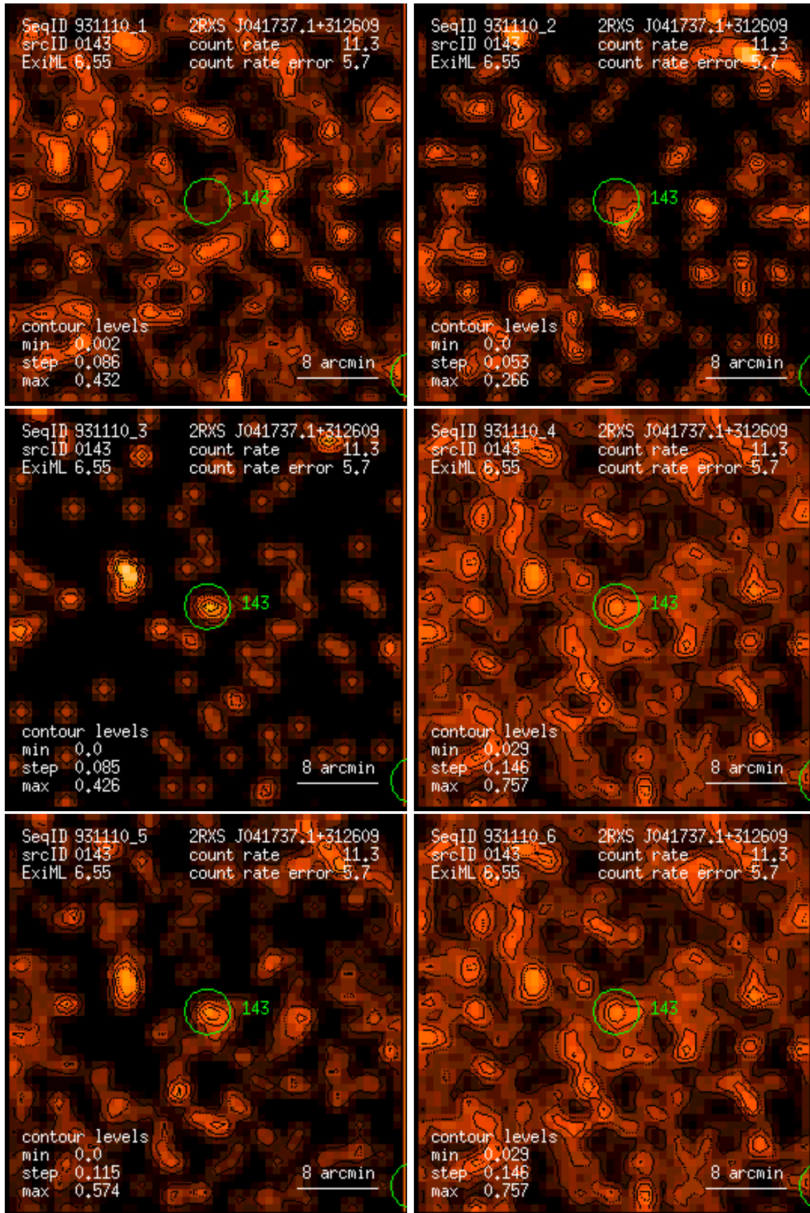
Figure 143: RASS 931110: detection 0143: band rate images, Gaussian filter: (1) PSPC channels 11 – 41, (2) 52 – 90, (3) 91 – 201, (4) 11 – 235, (5) 52 – 201, (6) 11 – 201. Broad band rates in counts/ks. Band rate contour levels in counts/ks/arcmin 2 .
