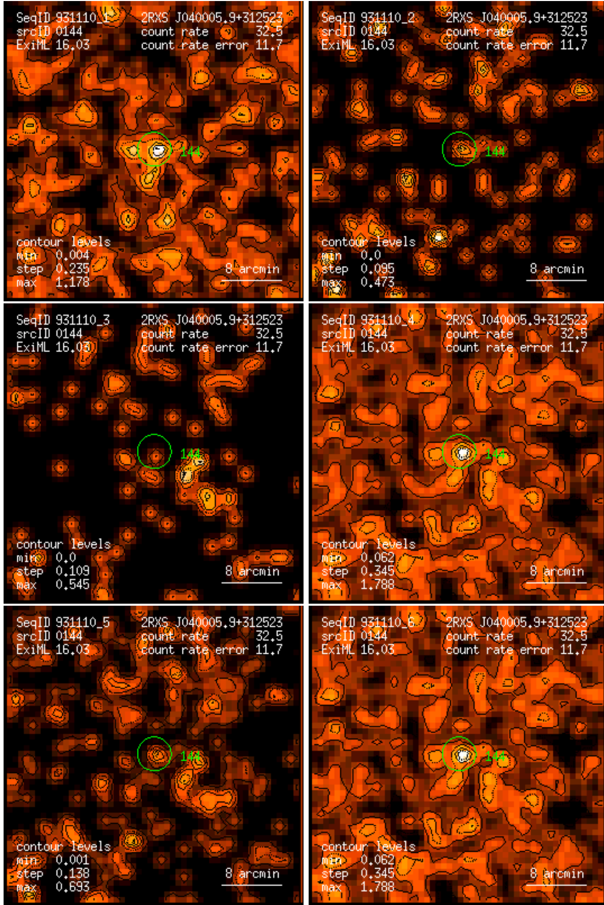
Figure 144: RASS 931110: detection 0144: band rate images, Gaussian filter: (1) PSPC channels 11 – 41, (2) 52 – 90, (3) 91 – 201, (4) 11 – 235, (5) 52 – 201, (6) 11 – 201. Broad band rates in counts/ks. Band rate contour levels in counts/ks/arcmin 2 .
