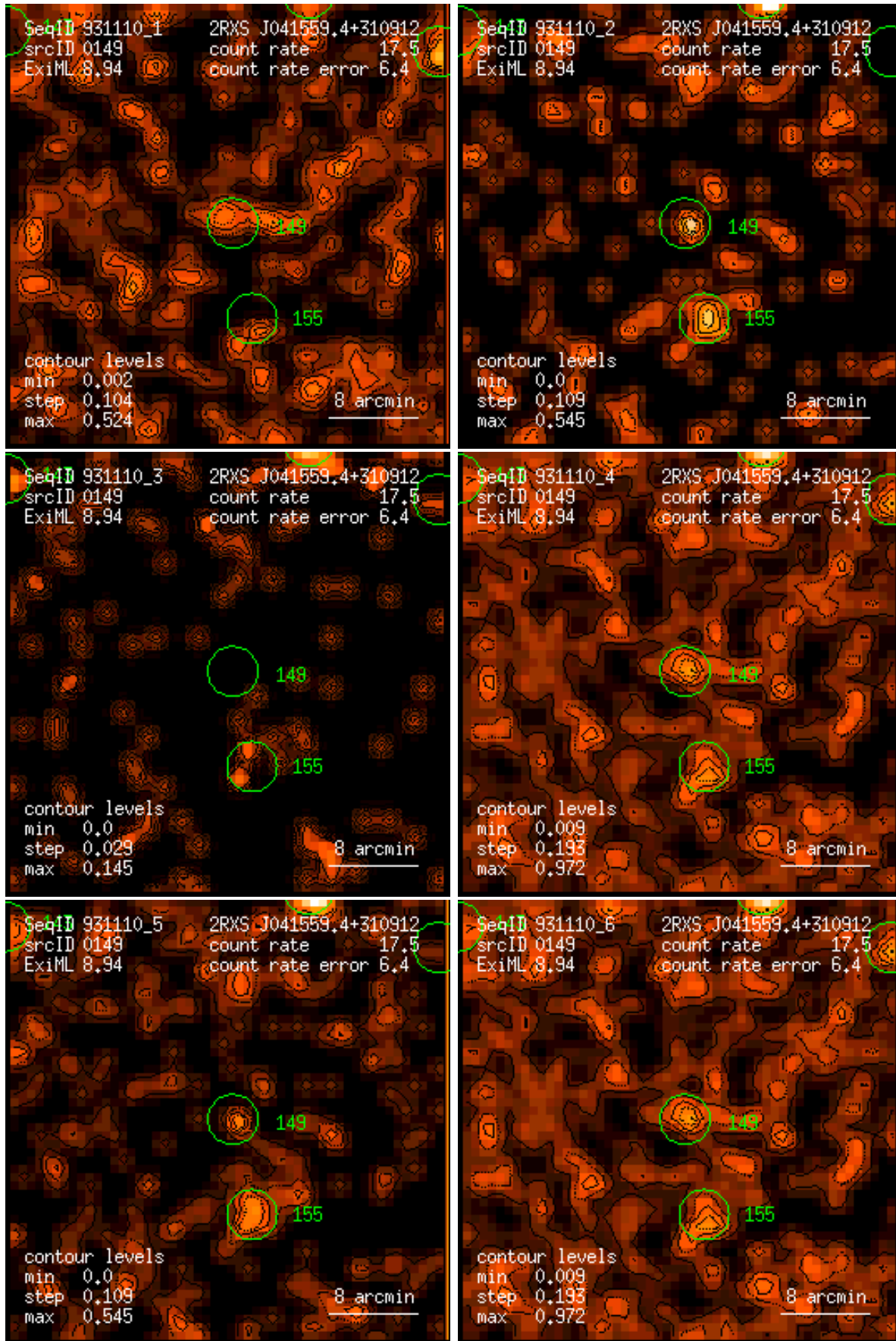
Figure 149: RASS 931110: detection 0149: band rate images, Gaussian filter: (1) PSPC channels 11 – 41, (2) 52 – 90, (3) 91 – 201, (4) 11 – 235, (5) 52 – 201, (6) 11 – 201. Broad band rates in counts/ks. Band rate contour levels in counts/ks/arcmin 2 .
