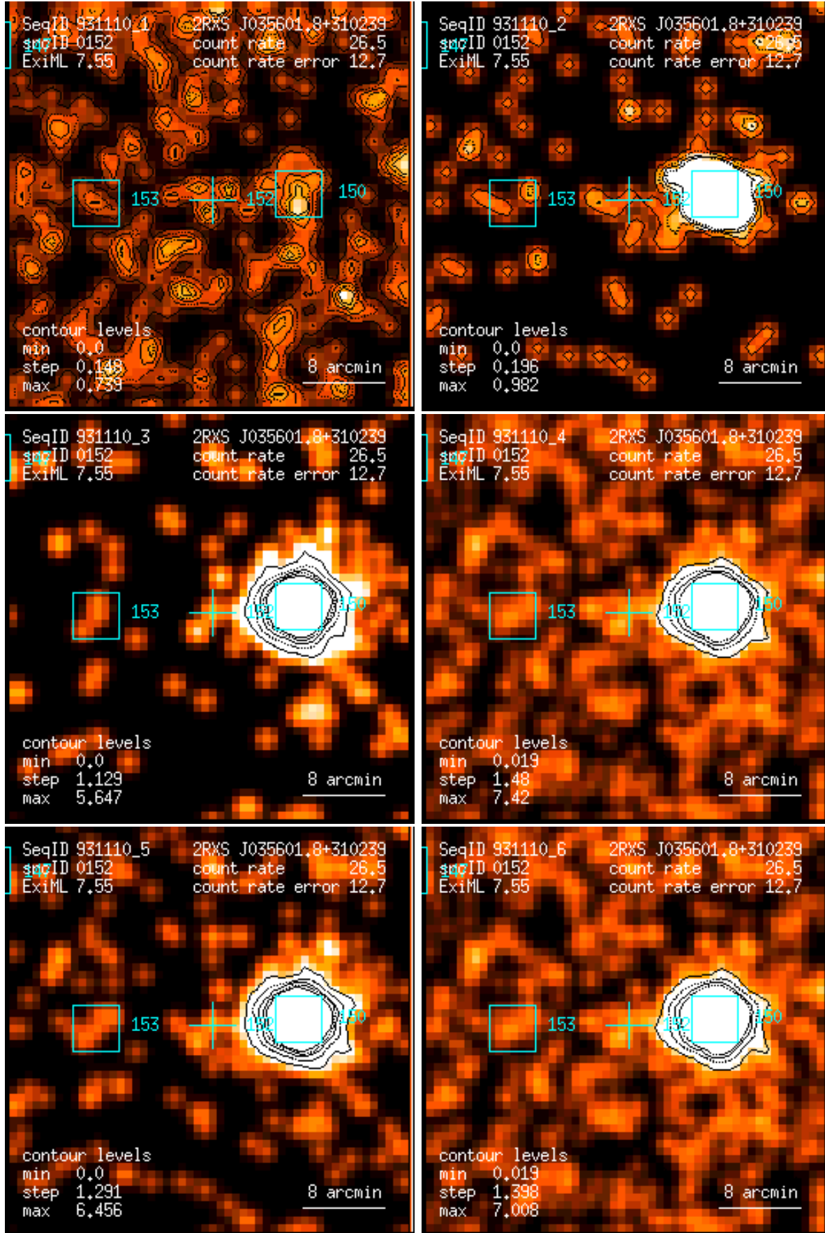
Figure 152: RASS 931110: detection 0152: band rate images, Gaussian filter: (1) PSPC channels 11 – 41, (2) 52 – 90, (3) 91 – 201, (4) 11 – 235, (5) 52 – 201, (6) 11 – 201. Broad band rates in counts/ks. Band rate contour levels in counts/ks/arcmin 2 .
