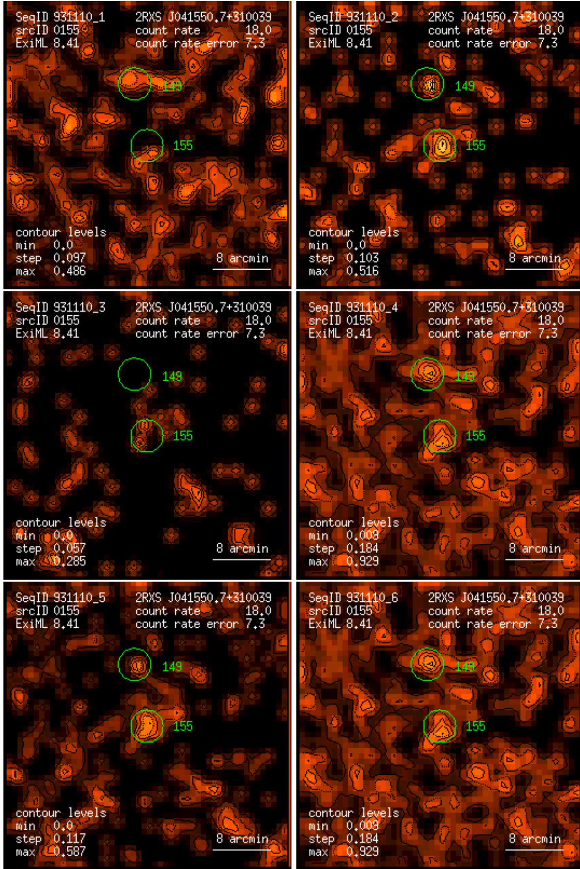
Figure 155: RASS 931110: detection 0155: band rate images, Gaussian filter: (1) PSPC channels 11 – 41, (2) 52 – 90, (3) 91 – 201, (4) 11 – 235, (5) 52 – 201, (6) 11 – 201. Broad band rates in counts/ks. Band rate contour levels in counts/ks/arcmin 2 .
