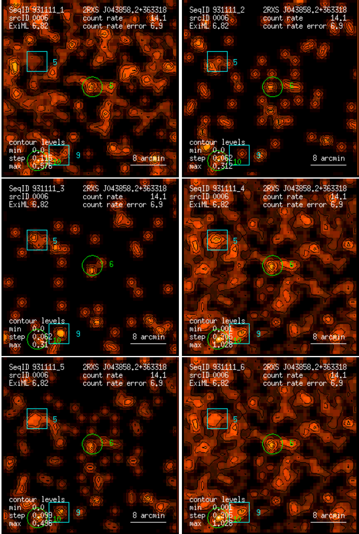
Figure 6: RASS 931111: detection 0006: band rate images, Gaussian filter: (1) PSPC channels 11 – 41, (2) 52 – 90, (3) 91 – 201, (4) 11 – 235, (5) 52 – 201, (6) 11 – 201. Broad band rates in counts/ks. Band rate contour levels in counts/ks/arcmin 2 .
