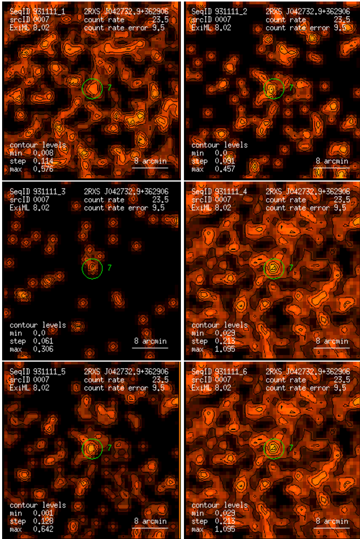
Figure 7: RASS 931111: detection 0007: band rate images, Gaussian filter: (1) PSPC channels 11 – 41, (2) 52 – 90, (3) 91 – 201, (4) 11 – 235, (5) 52 – 201, (6) 11 – 201. Broad band rates in counts/ks. Band rate contour levels in counts/ks/arcmin 2 .
