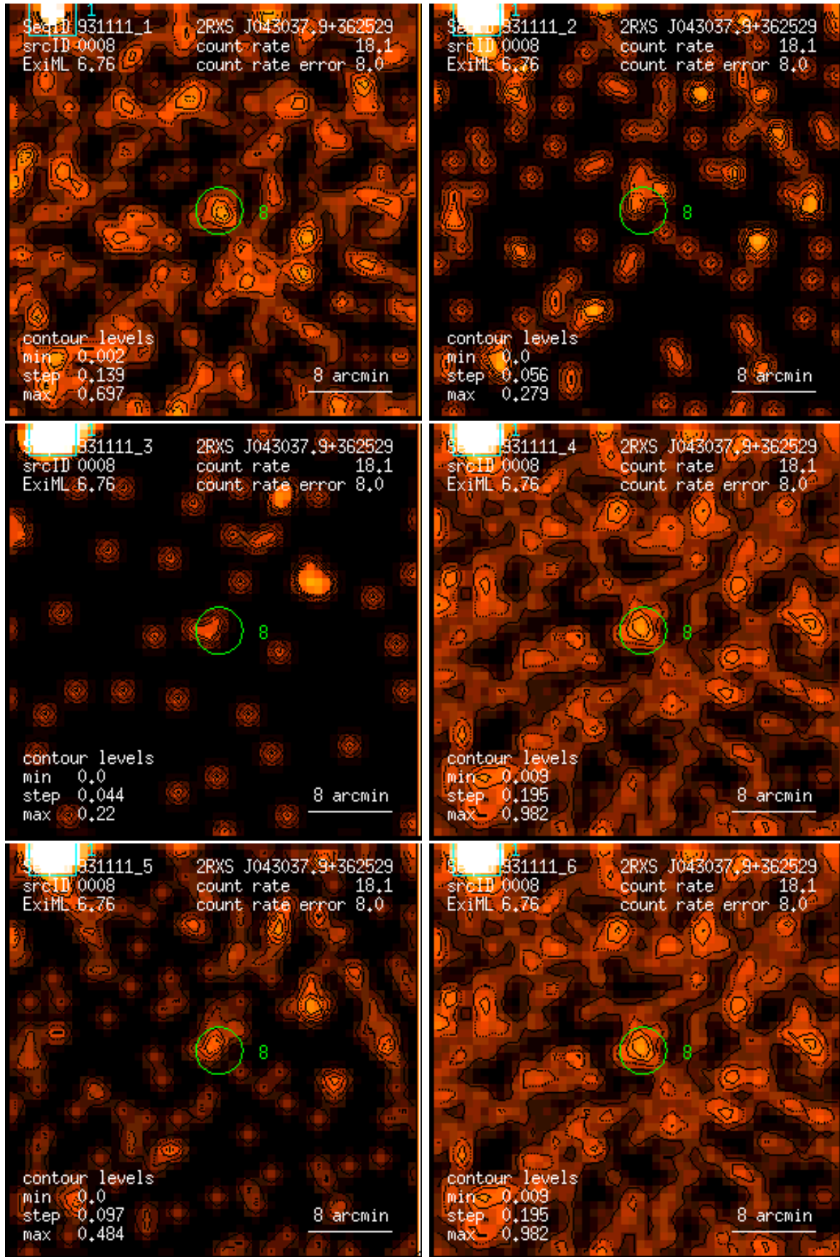
Figure 8: RASS 931111: detection 0008: band rate images, Gaussian filter: (1) PSPC channels 11 – 41, (2) 52 – 90, (3) 91 – 201, (4) 11 – 235, (5) 52 – 201, (6) 11 – 201. Broad band rates in counts/ks. Band rate contour levels in counts/ks/arcmin 2 .
