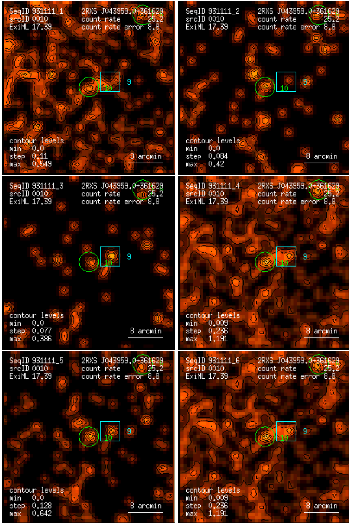
Figure 10: RASS 931111: detection 0010: band rate images, Gaussian filter: (1) PSPC channels 11 – 41, (2) 52 – 90, (3) 91 – 201, (4) 11 – 235, (5) 52 – 201, (6) 11 – 201. Broad band rates in counts/ks. Band rate contour levels in counts/ks/arcmin 2 .
