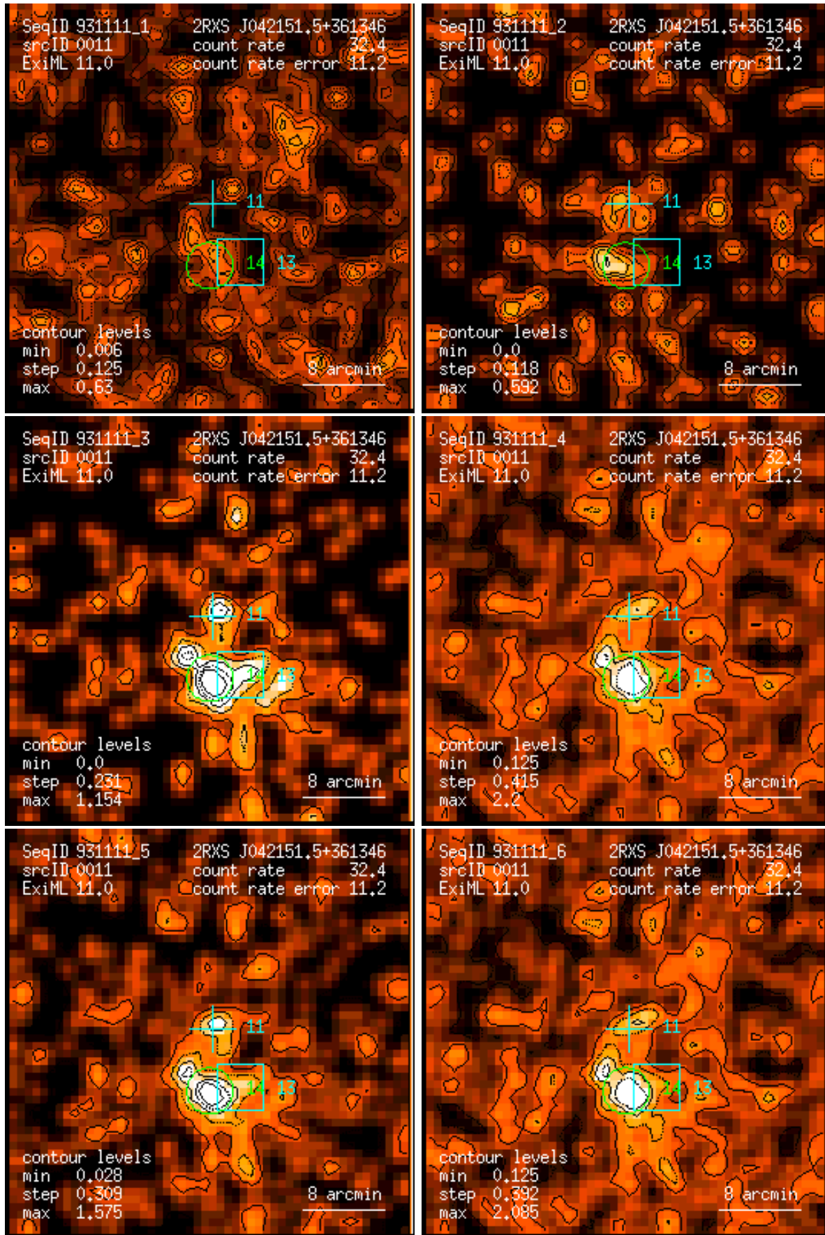
Figure 11: RASS 931111: detection 0011: band rate images, Gaussian filter: (1) PSPC channels 11 – 41, (2) 52 – 90, (3) 91 – 201, (4) 11 – 235, (5) 52 – 201, (6) 11 – 201. Broad band rates in counts/ks. Band rate contour levels in counts/ks/arcmin 2 .
