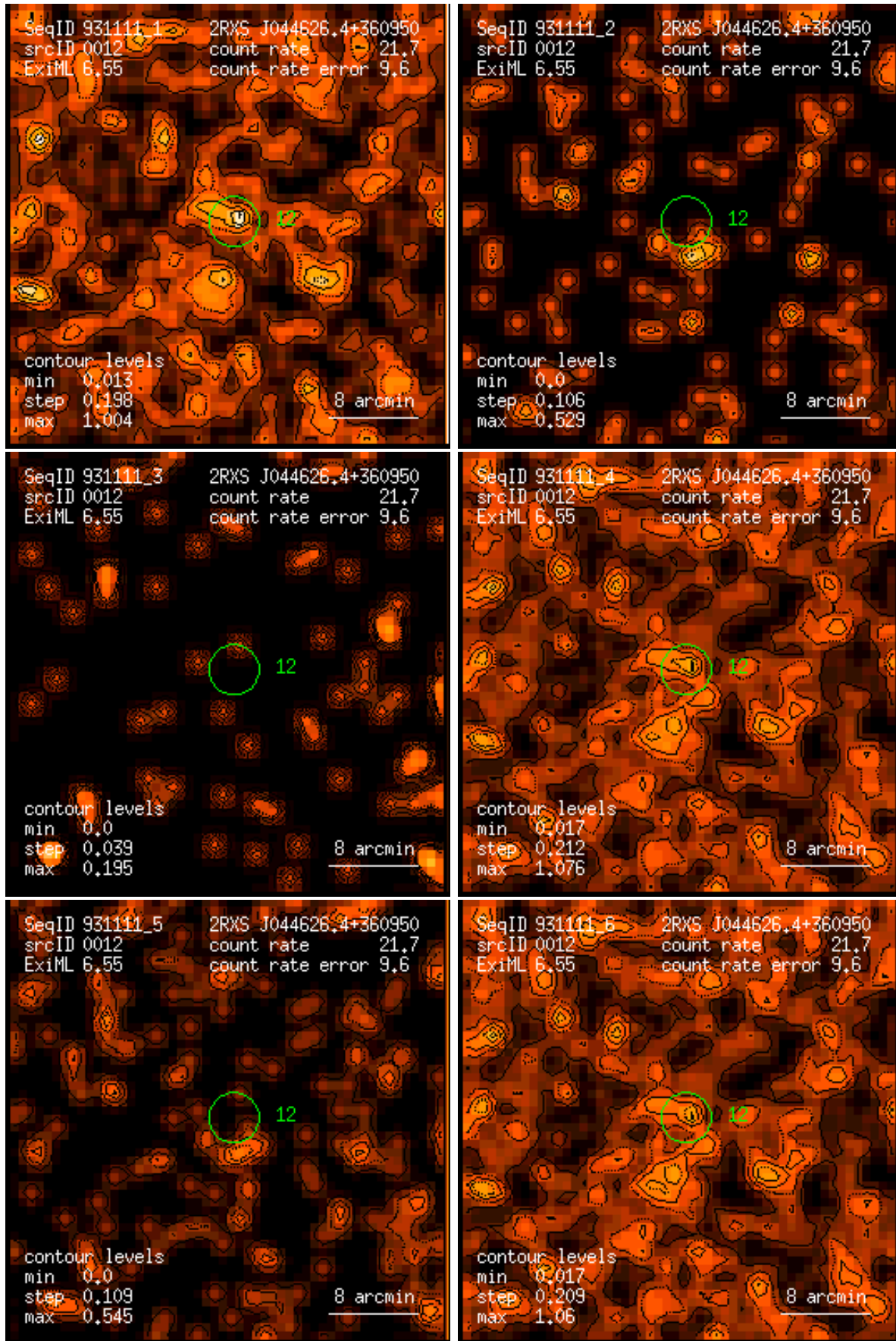
Figure 12: RASS 931111: detection 0012: band rate images, Gaussian filter: (1) PSPC channels 11 – 41, (2) 52 – 90, (3) 91 – 201, (4) 11 – 235, (5) 52 – 201, (6) 11 – 201. Broad band rates in counts/ks. Band rate contour levels in counts/ks/arcmin 2 .
