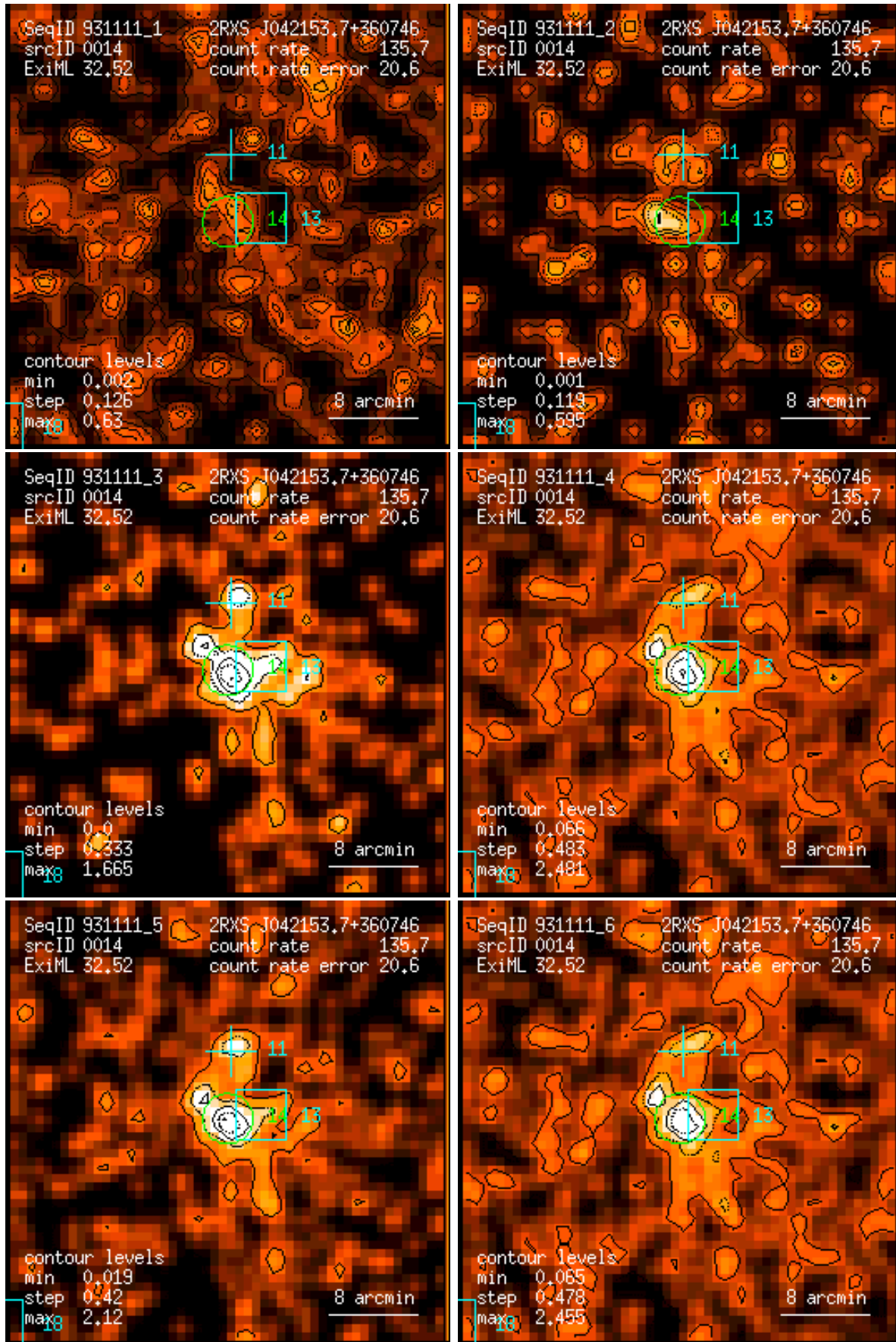
Figure 14: RASS 931111: detection 0014: band rate images, Gaussian filter: (1) PSPC channels 11 – 41, (2) 52 – 90, (3) 91 – 201, (4) 11 – 235, (5) 52 – 201, (6) 11 – 201. Broad band rates in counts/ks. Band rate contour levels in counts/ks/arcmin 2 .
