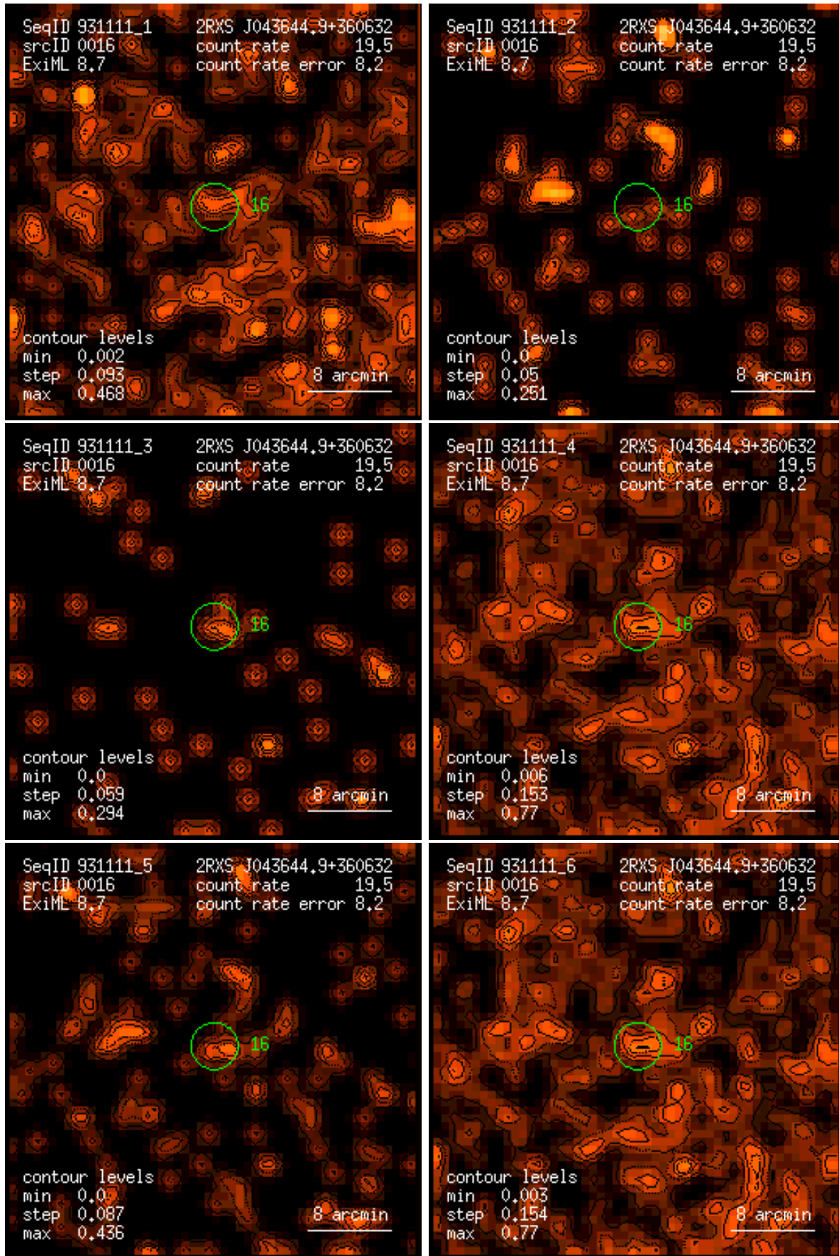
Figure 16: RASS 931111: detection 0016: band rate images, Gaussian filter: (1) PSPC channels 11 – 41, (2) 52 – 90, (3) 91 – 201, (4) 11 – 235, (5) 52 – 201, (6) 11 – 201. Broad band rates in counts/ks. Band rate contour levels in counts/ks/arcmin 2 .
