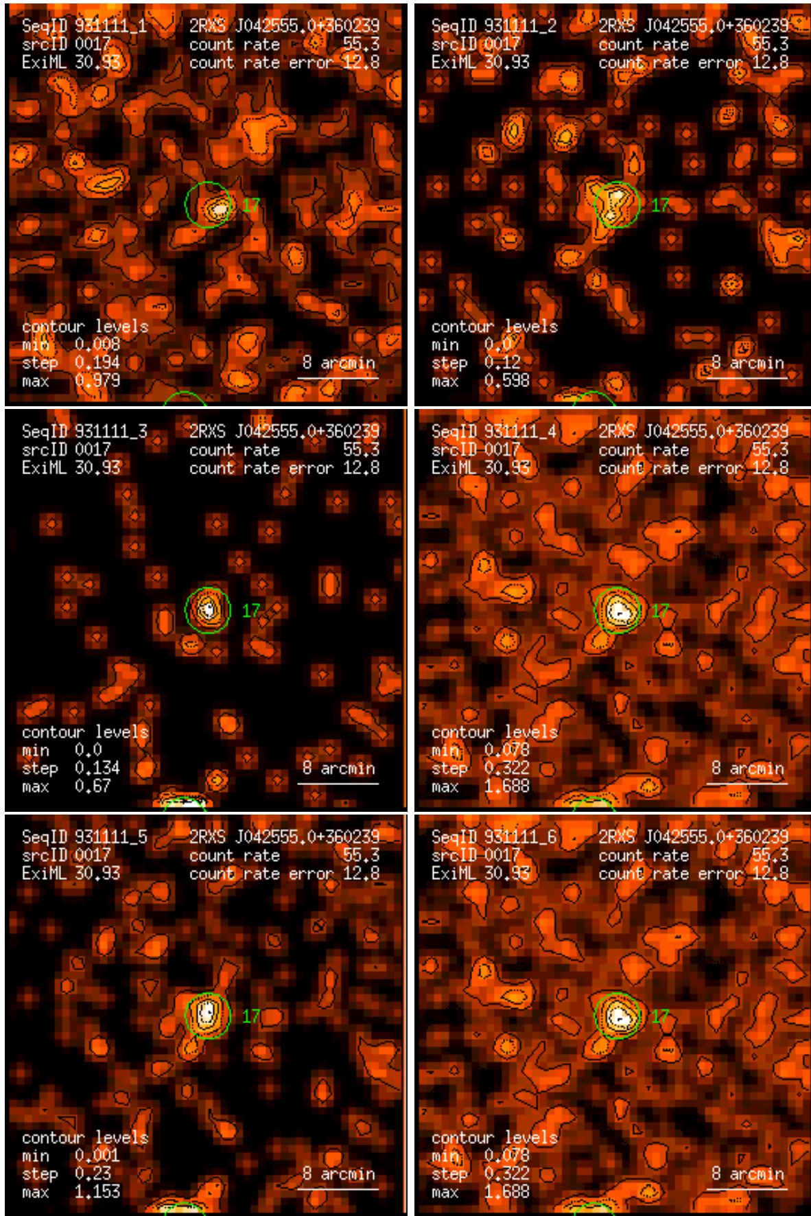
Figure 17: RASS 931111: detection 0017: band rate images, Gaussian filter: (1) PSPC channels 11 – 41, (2) 52 – 90, (3) 91 – 201, (4) 11 – 235, (5) 52 – 201, (6) 11 – 201. Broad band rates in counts/ks. Band rate contour levels in counts/ks/arcmin 2 .
