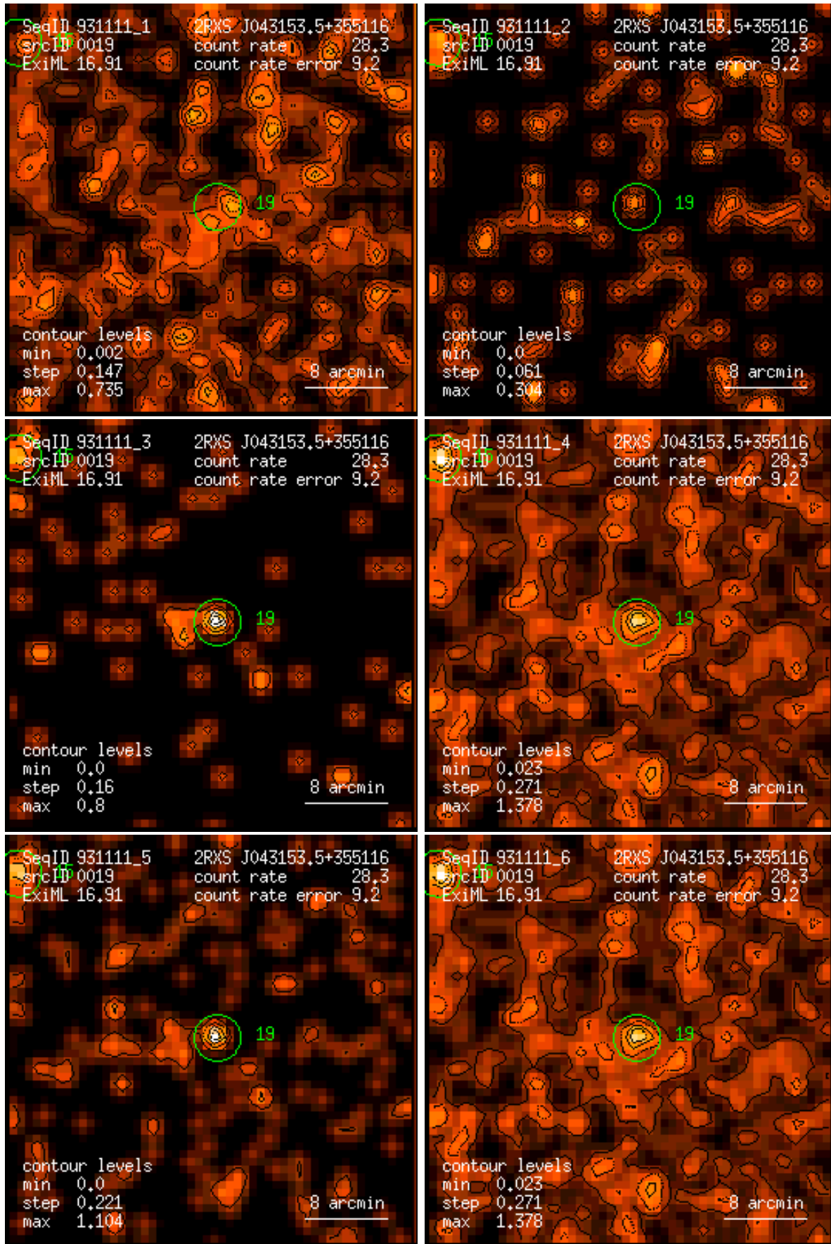
Figure 19: RASS 931111: detection 0019: band rate images, Gaussian filter: (1) PSPC channels 11 – 41, (2) 52 – 90, (3) 91 – 201, (4) 11 – 235, (5) 52 – 201, (6) 11 – 201. Broad band rates in counts/ks. Band rate contour levels in counts/ks/arcmin 2 .
