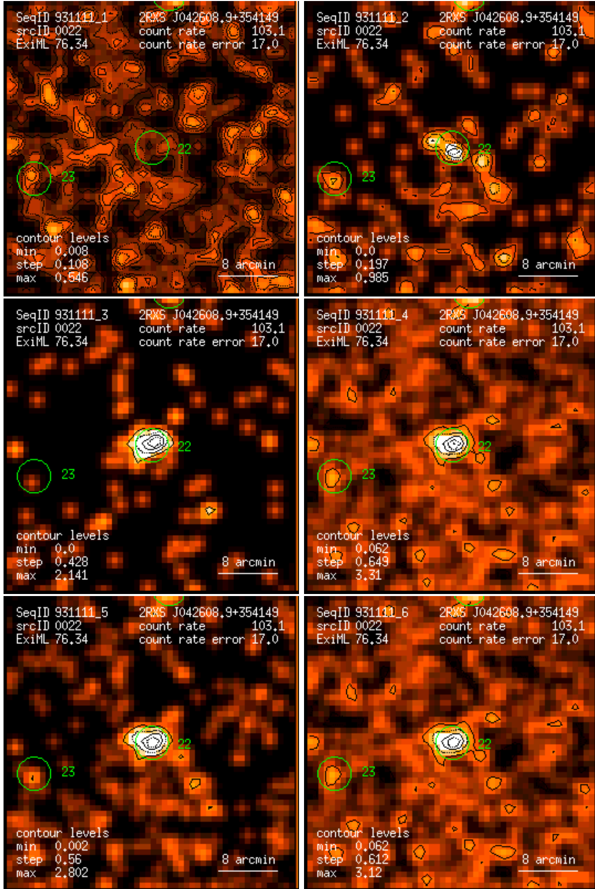
Figure 22: RASS 931111: detection 0022: band rate images, Gaussian filter: (1) PSPC channels 11 – 41, (2) 52 – 90, (3) 91 – 201, (4) 11 – 235, (5) 52 – 201, (6) 11 – 201. Broad band rates in counts/ks. Band rate contour levels in counts/ks/arcmin 2 .
