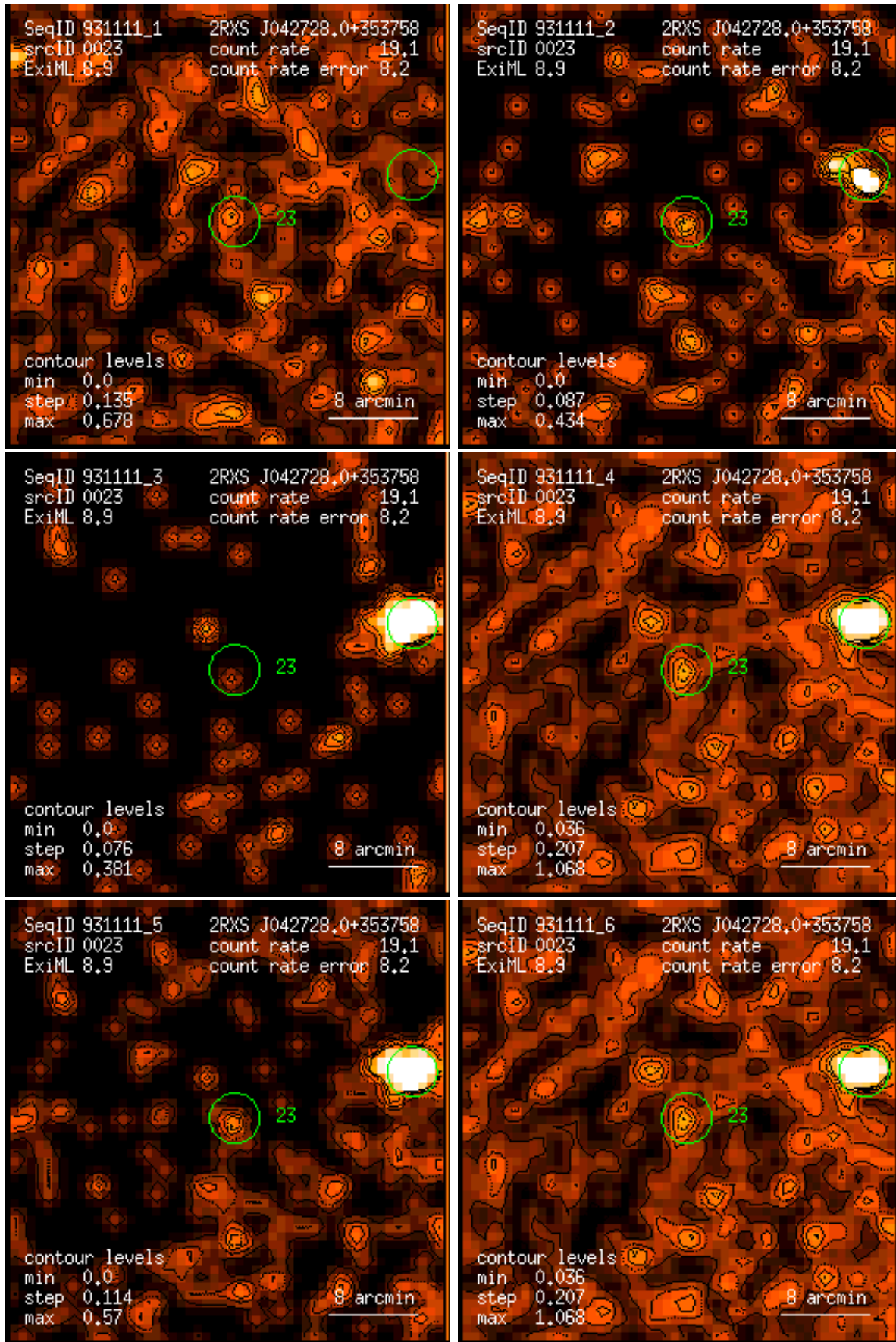
Figure 23: RASS 931111: detection 0023: band rate images, Gaussian filter: (1) PSPC channels 11 – 41, (2) 52 – 90, (3) 91 – 201, (4) 11 – 235, (5) 52 – 201, (6) 11 – 201. Broad band rates in counts/ks. Band rate contour levels in counts/ks/arcmin 2 .
