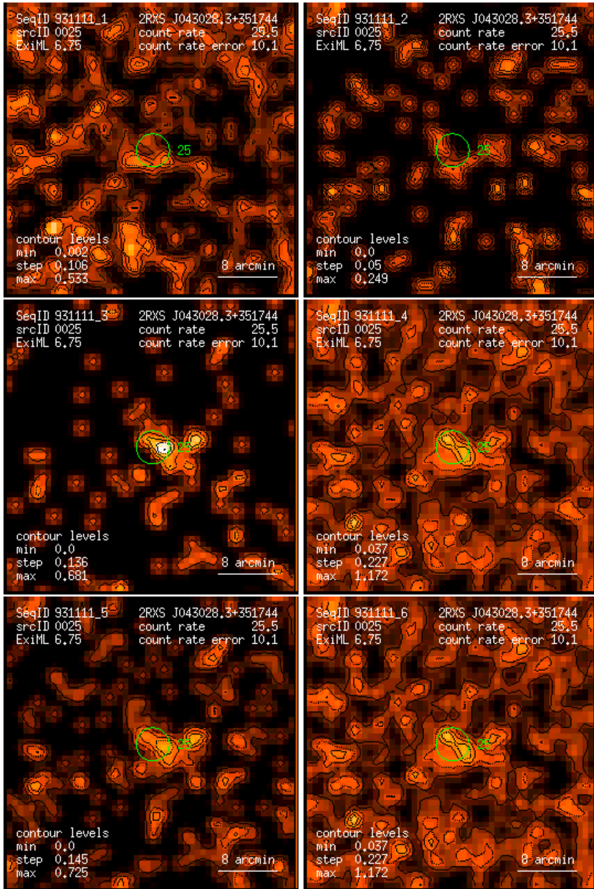
Figure 25: RASS 931111: detection 0025: band rate images, Gaussian filter: (1) PSPC channels 11 – 41, (2) 52 – 90, (3) 91 – 201, (4) 11 – 235, (5) 52 – 201, (6) 11 – 201. Broad band rates in counts/ks. Band rate contour levels in counts/ks/arcmin 2 .
