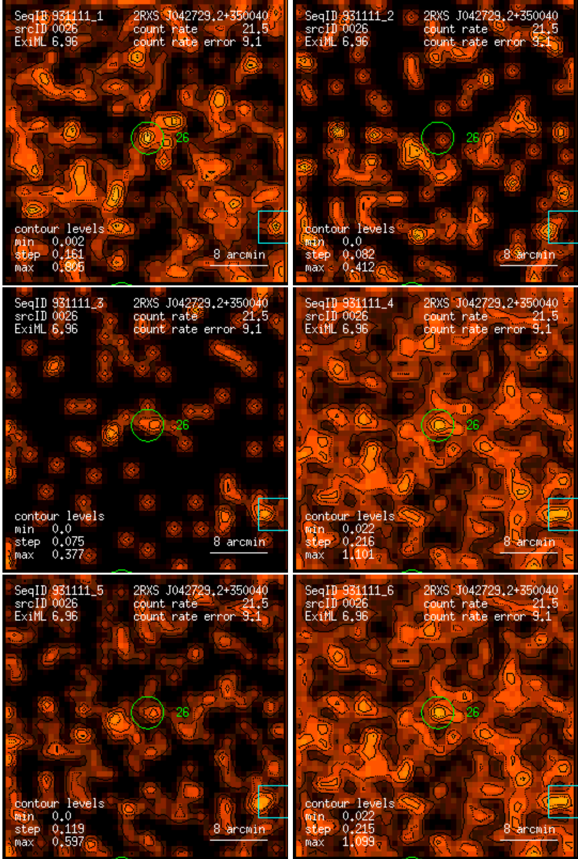
Figure 26: RASS 931111: detection 0026: band rate images, Gaussian filter: (1) PSPC channels 11 – 41, (2) 52 – 90, (3) 91 – 201, (4) 11 – 235, (5) 52 – 201, (6) 11 – 201. Broad band rates in counts/ks. Band rate contour levels in counts/ks/arcmin 2 .
