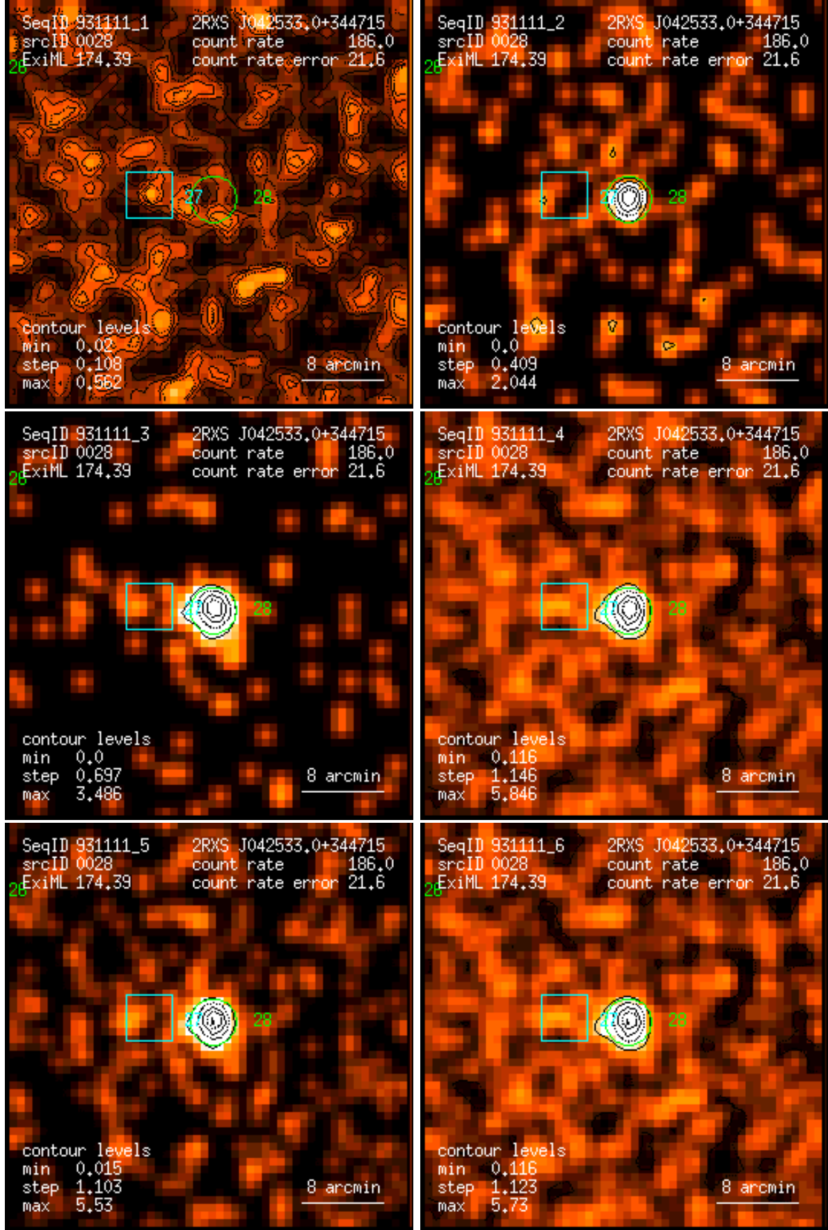
Figure 28: RASS 931111: detection 0028: band rate images, Gaussian filter: (1) PSPC channels 11 – 41, (2) 52 – 90, (3) 91 – 201, (4) 11 – 235, (5) 52 – 201, (6) 11 – 201. Broad band rates in counts/ks. Band rate contour levels in counts/ks/arcmin 2 .
