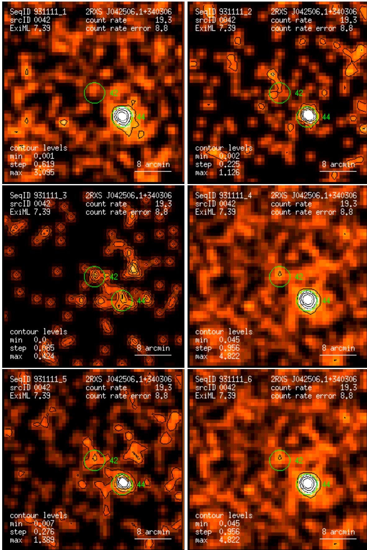
Figure 42: RASS 931111: detection 0042: band rate images, Gaussian filter: (1) PSPC channels 11 – 41, (2) 52 – 90, (3) 91 – 201, (4) 11 – 235, (5) 52 – 201, (6) 11 – 201. Broad band rates in counts/ks. Band rate contour levels in counts/ks/arcmin 2 .
