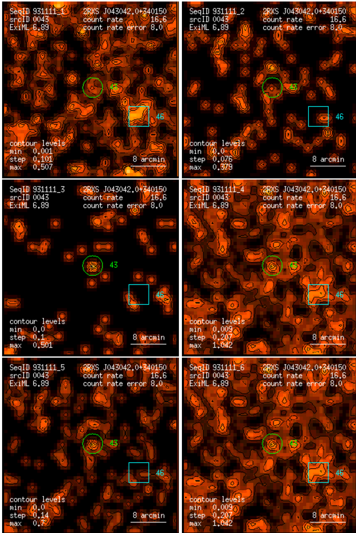
Figure 43: RASS 931111: detection 0043: band rate images, Gaussian filter: (1) PSPC channels 11 – 41, (2) 52 – 90, (3) 91 – 201, (4) 11 – 235, (5) 52 – 201, (6) 11 – 201. Broad band rates in counts/ks. Band rate contour levels in counts/ks/arcmin 2 .
