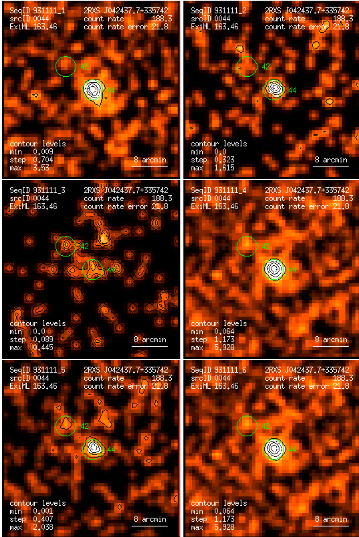
Figure 44: RASS 931111: detection 0044: band rate images, Gaussian filter: (1) PSPC channels 11 – 41, (2) 52 – 90, (3) 91 – 201, (4) 11 – 235, (5) 52 – 201, (6) 11 – 201. Broad band rates in counts/ks. Band rate contour levels in counts/ks/arcmin 2 .
