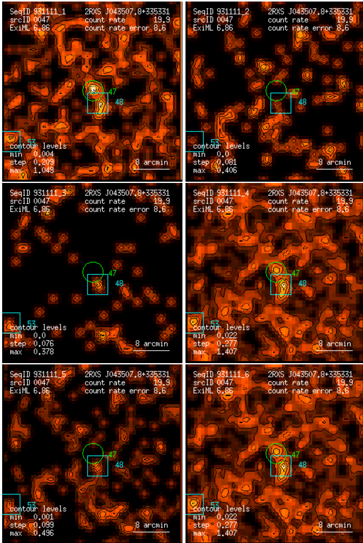
Figure 47: RASS 931111: detection 0047: band rate images, Gaussian filter: (1) PSPC channels 11 – 41, (2) 52 – 90, (3) 91 – 201, (4) 11 – 235, (5) 52 – 201, (6) 11 – 201. Broad band rates in counts/ks. Band rate contour levels in counts/ks/arcmin 2 .
