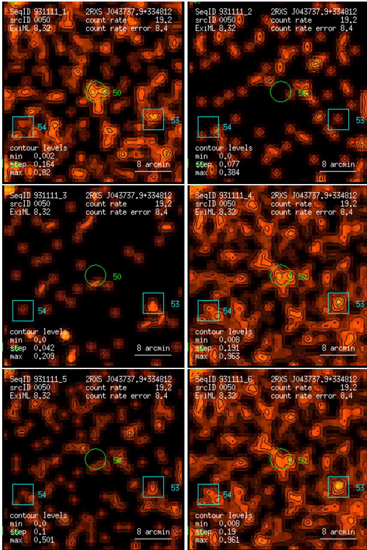
Figure 50: RASS 931111: detection 0050: band rate images, Gaussian filter: (1) PSPC channels 11 – 41, (2) 52 – 90, (3) 91 – 201, (4) 11 – 235, (5) 52 – 201, (6) 11 – 201. Broad band rates in counts/ks. Band rate contour levels in counts/ks/arcmin 2 .
