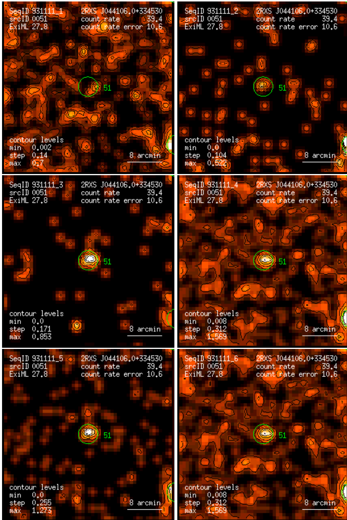
Figure 51: RASS 931111: detection 0051: band rate images, Gaussian filter: (1) PSPC channels 11 – 41, (2) 52 – 90, (3) 91 – 201, (4) 11 – 235, (5) 52 – 201, (6) 11 – 201. Broad band rates in counts/ks. Band rate contour levels in counts/ks/arcmin 2 .
