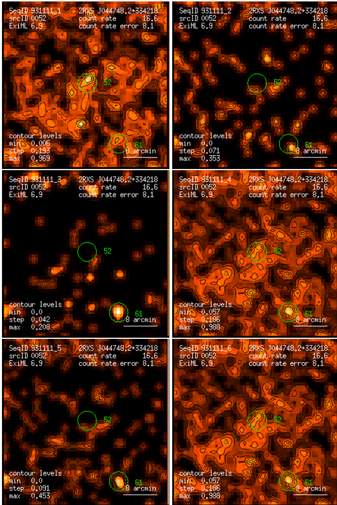
Figure 52: RASS 931111: detection 0052: band rate images, Gaussian filter: (1) PSPC channels 11 – 41, (2) 52 – 90, (3) 91 – 201, (4) 11 – 235, (5) 52 – 201, (6) 11 – 201. Broad band rates in counts/ks. Band rate contour levels in counts/ks/arcmin 2 .
