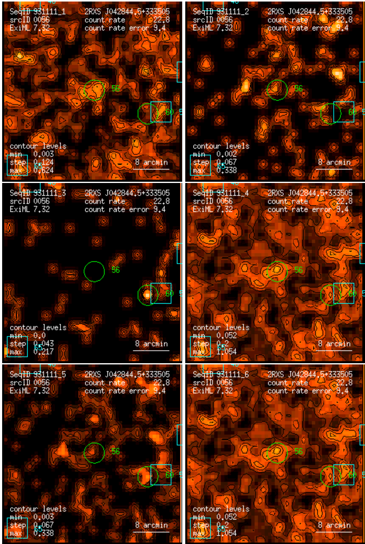
Figure 56: RASS 931111: detection 0056: band rate images, Gaussian filter: (1) PSPC channels 11 – 41, (2) 52 – 90, (3) 91 – 201, (4) 11 – 235, (5) 52 – 201, (6) 11 – 201. Broad band rates in counts/ks. Band rate contour levels in counts/ks/arcmin 2 .
