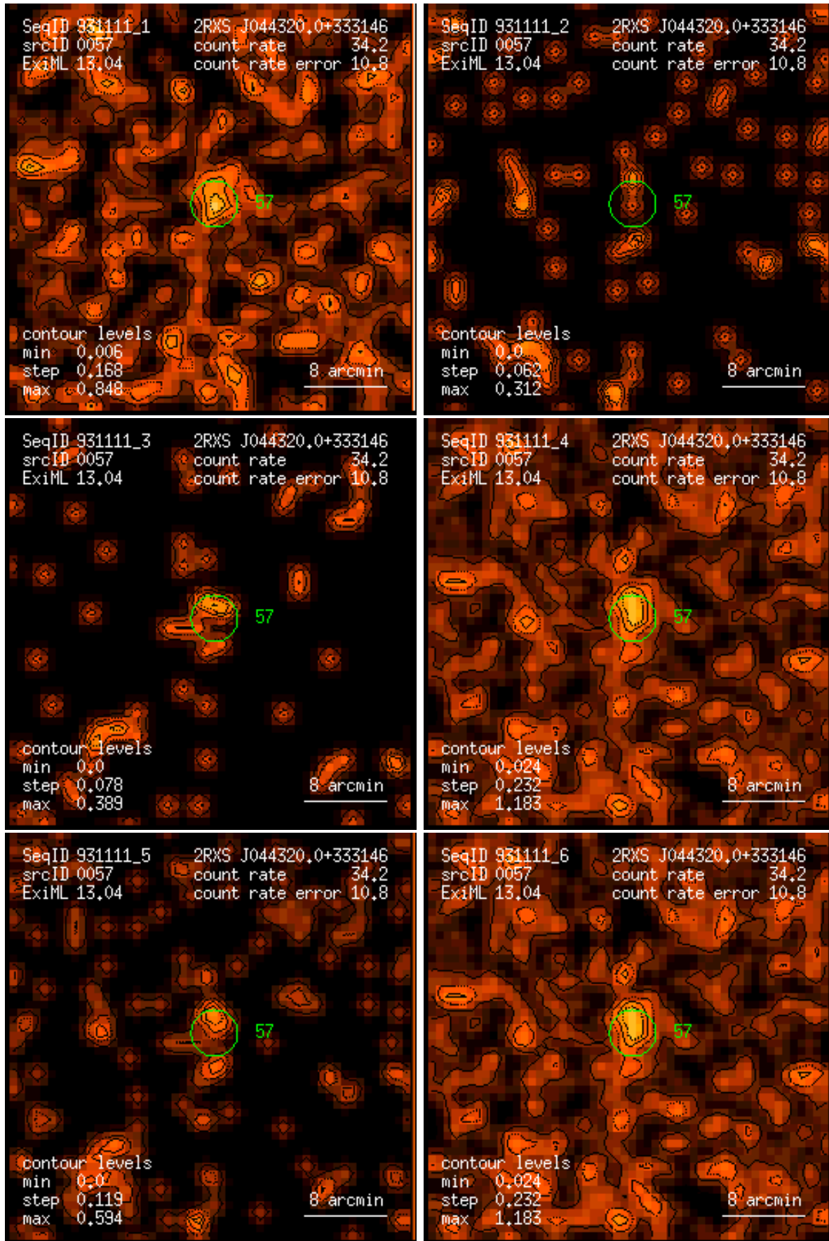
Figure 57: RASS 931111: detection 0057: band rate images, Gaussian filter: (1) PSPC channels 11 – 41, (2) 52 – 90, (3) 91 – 201, (4) 11 – 235, (5) 52 – 201, (6) 11 – 201. Broad band rates in counts/ks. Band rate contour levels in counts/ks/arcmin 2 .
