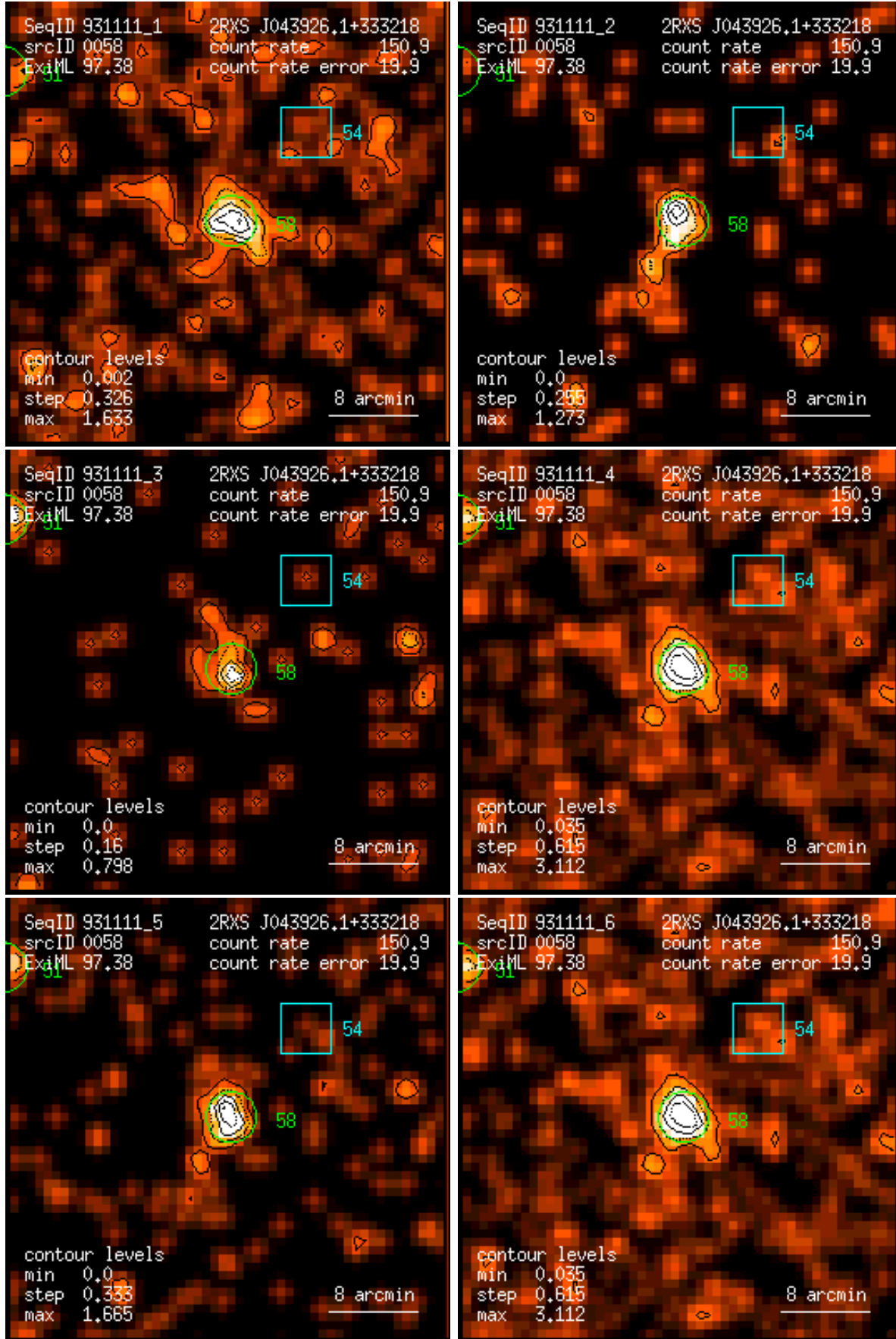
Figure 58: RASS 931111: detection 0058: band rate images, Gaussian filter: (1) PSPC channels 11 – 41, (2) 52 – 90, (3) 91 – 201, (4) 11 – 235, (5) 52 – 201, (6) 11 – 201. Broad band rates in counts/ks. Band rate contour levels in counts/ks/arcmin 2 .
