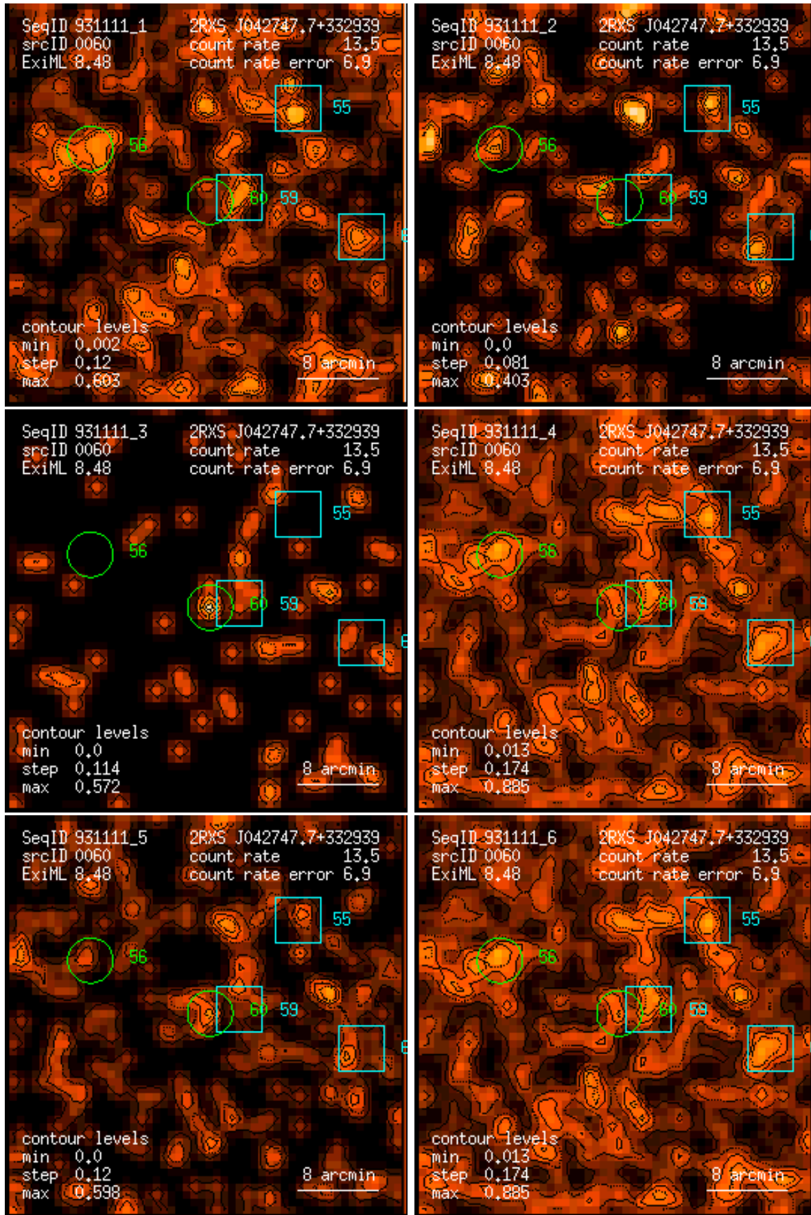
Figure 60: RASS 931111: detection 0060: band rate images, Gaussian filter: (1) PSPC channels 11 – 41, (2) 52 – 90, (3) 91 – 201, (4) 11 – 235, (5) 52 – 201, (6) 11 – 201. Broad band rates in counts/ks. Band rate contour levels in counts/ks/arcmin 2 .
